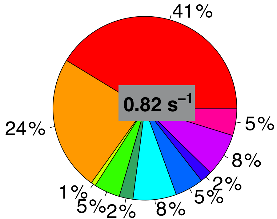
Observations (SH)
