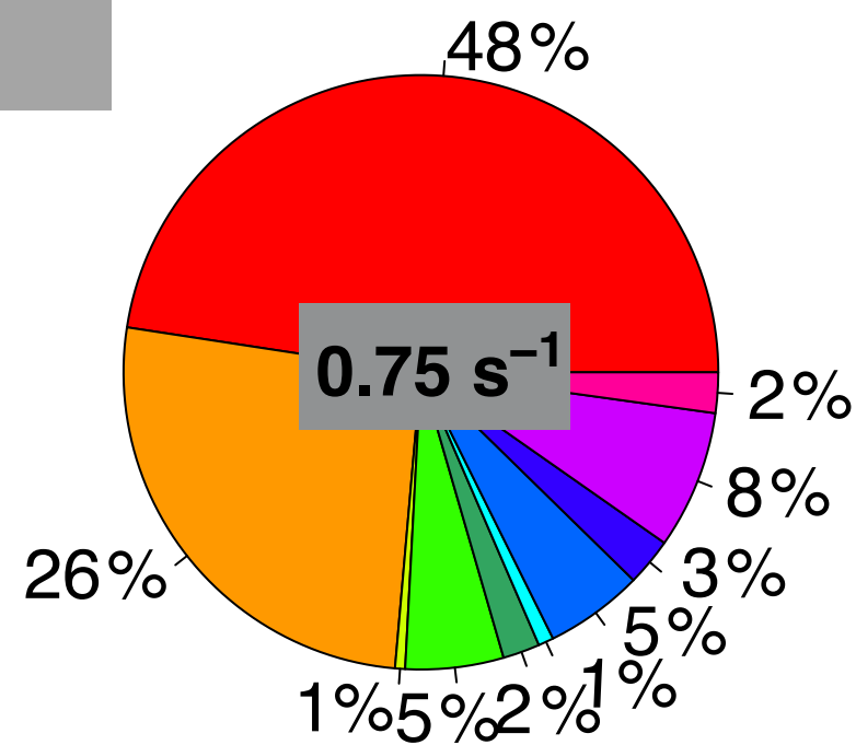
Model (SH)
