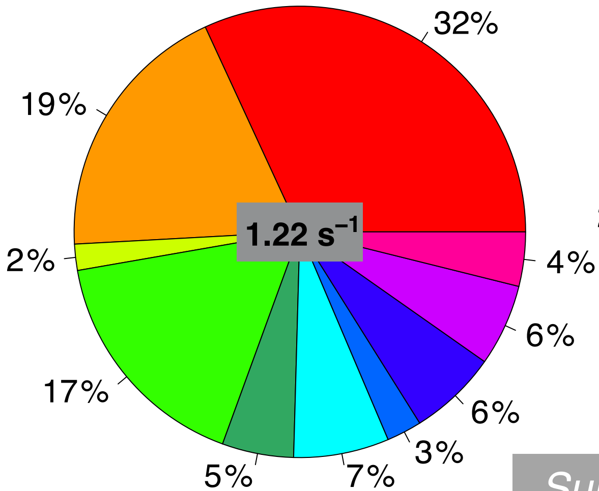
Observations (NH)
