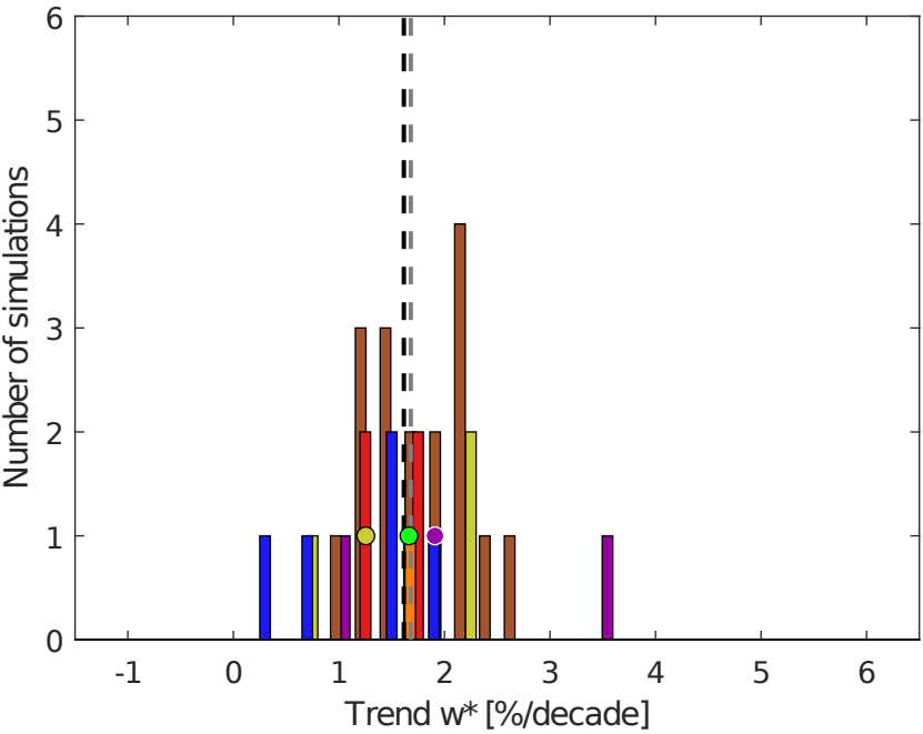
(c) w^* 70 hPa Trend, 1975-2014
