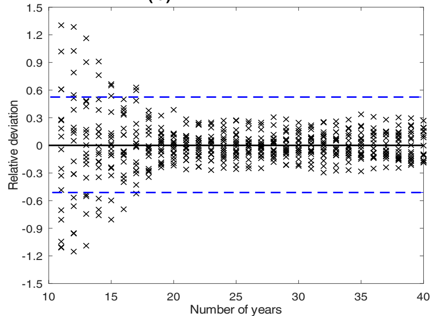
(b) AoA 30 hPa Trend
