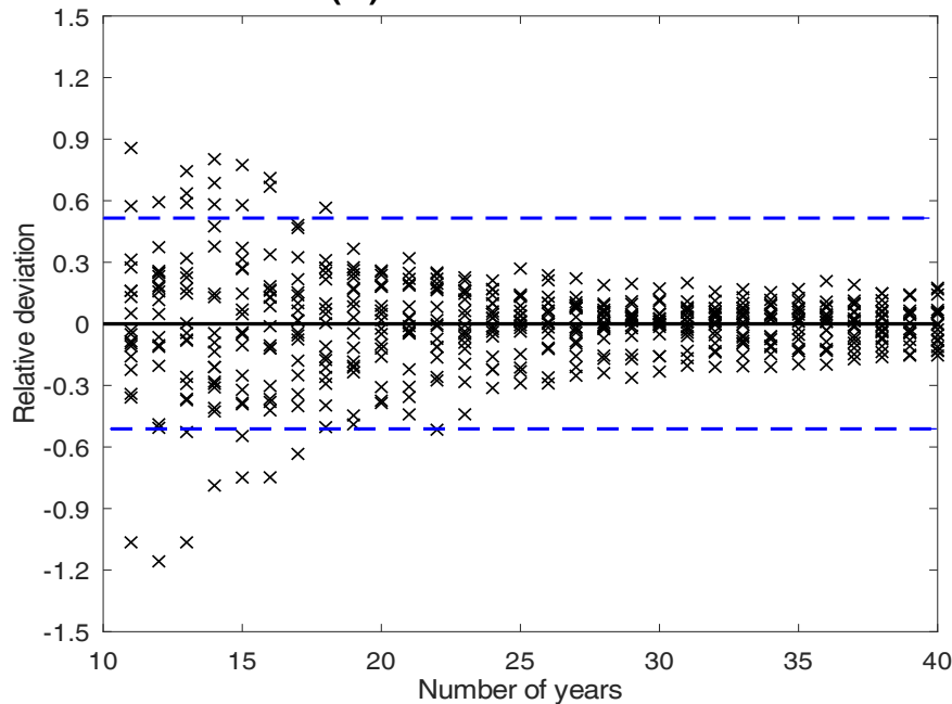
(a) AoA 80 hPa Trend
