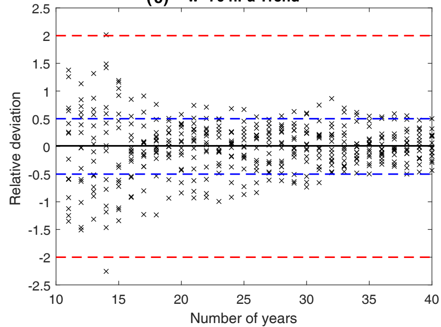
(c) w^* 70 hPa Trend
