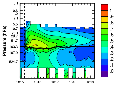
SOCOL-AER band
