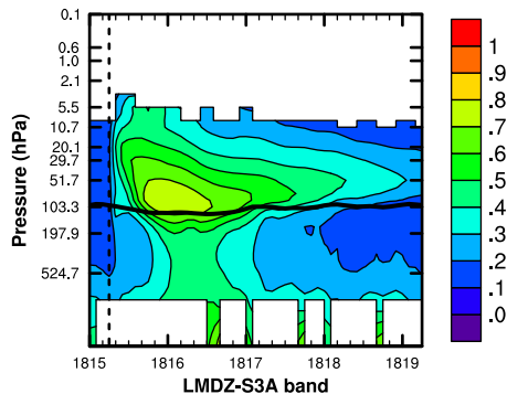
SOCOL-AER point
