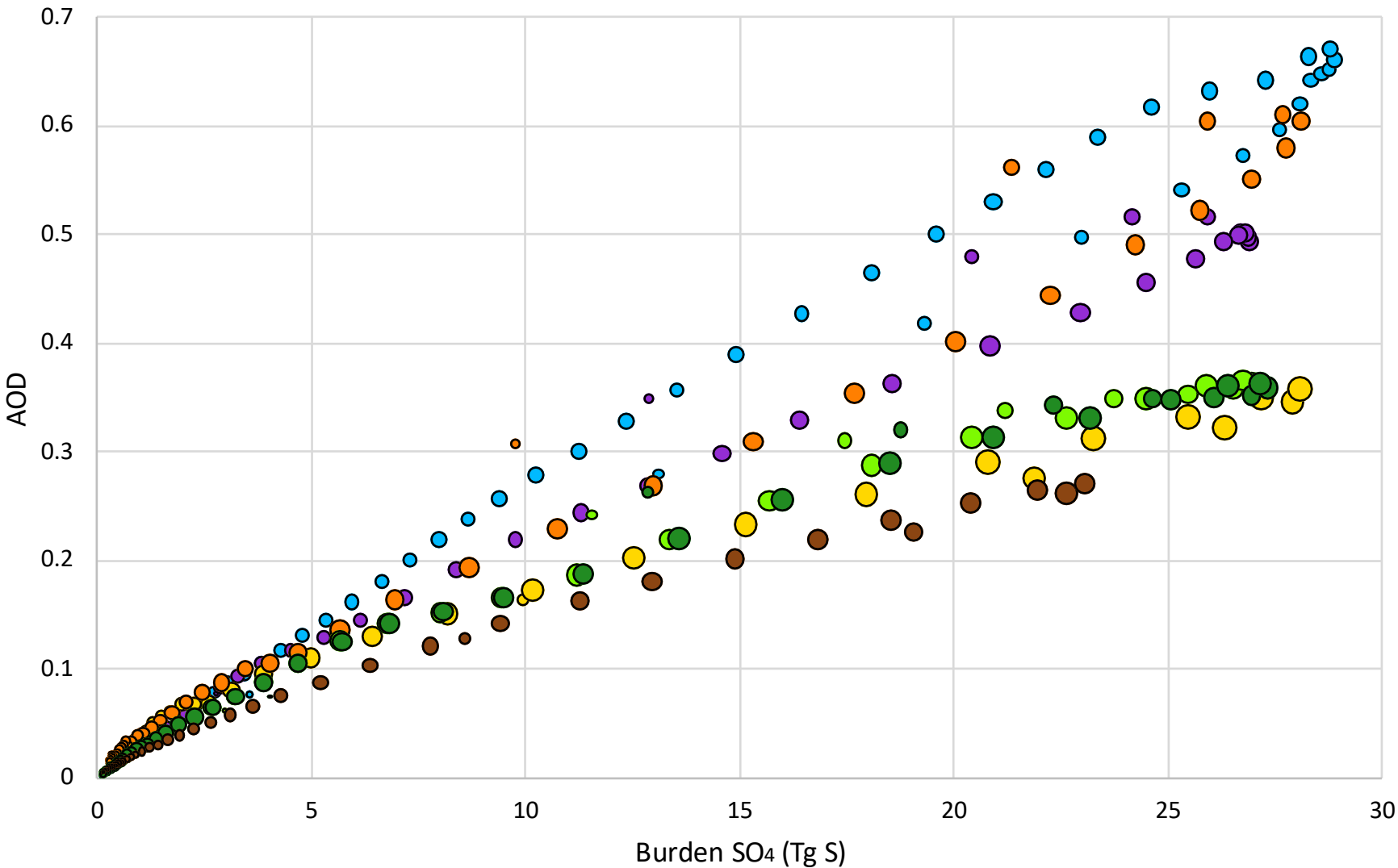
Global Stratospheric AOD vs. Sulfate Burden
