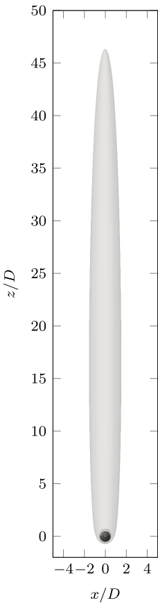
(a) Re = 75
