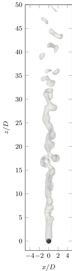
(b) Re = 600
