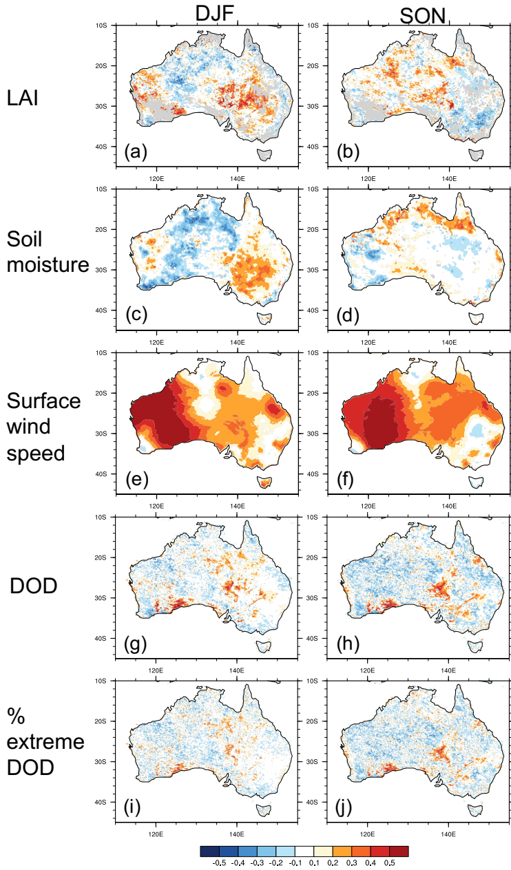
Figure S1 Autocorrelation of the seasonal mean key dust and environmental variables averaged for September-February dust season at one year lag during 2003-2019.
