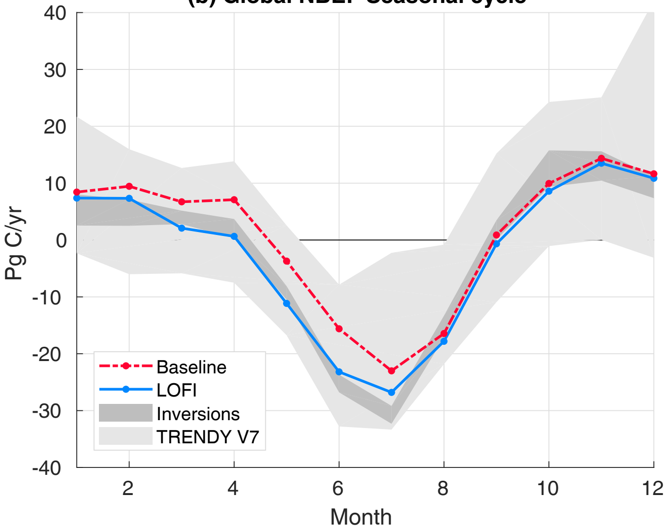
(b) Global NBE: Seasonal cycle
