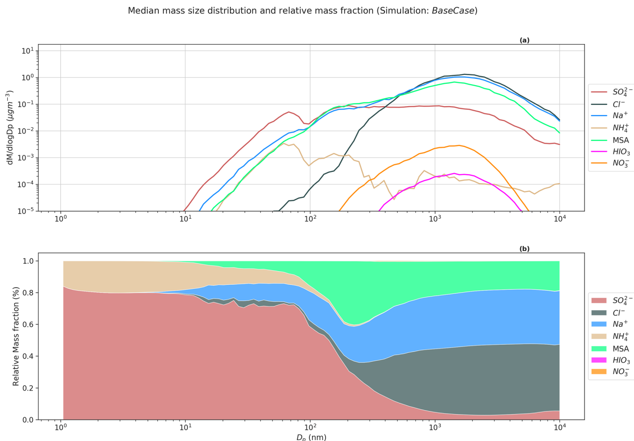
Figure 5. Simulated median mass size distribution for BaseCase simulations. The upper panel (a) shows the median mass size distribution for compounds \text{Cl}^- , \text{Na}^+ , MSA, \text{SO}_4^{2-} , \text{NH}_4^+ , \text{HIO}_3 , and \text{NO}_3^- for the entire size distribution ranging from 1.07 nm–10 \mu\text{m} . The lower panel (b) shows the relative mass fractions or contribution of compounds \text{Cl}^- , \text{Na}^+ , MSA, \text{SO}_4^{2-} , \text{NH}_4^+ , \text{HIO}_3 , and \text{NO}_3^- to total non-refractory PM at different sizes.
