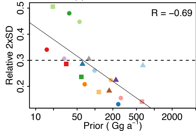
(c) Prior emissions
