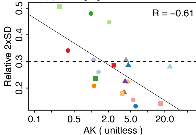
(e) Averaging kernel sensitivities
