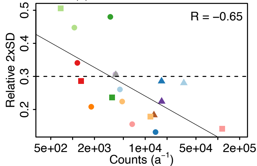
(a) TROPOMI obs counts
