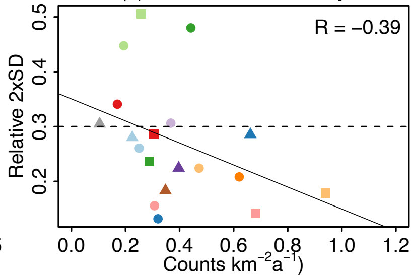
(b) TROPOMI obs density
