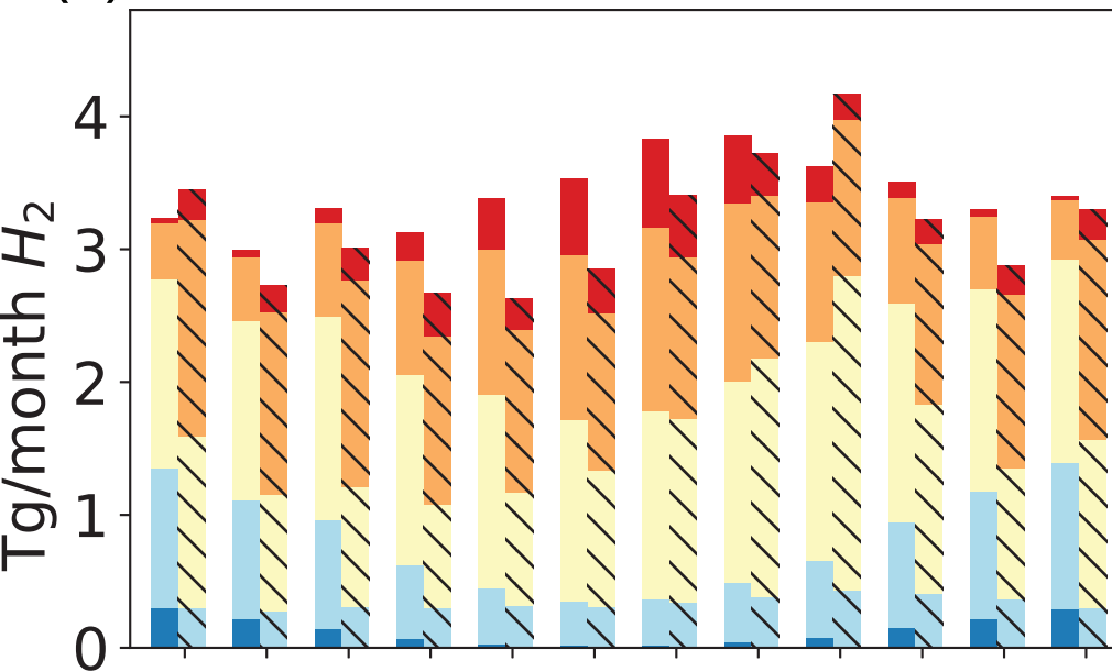
(c) 2015 ChemLoss DryDep
