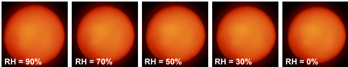
(a) \beta -caryophyllene/ O_3 SOA (O/C = 0.40) + \alpha -pinene/ O_3 SOA (O/C = 0.50)
