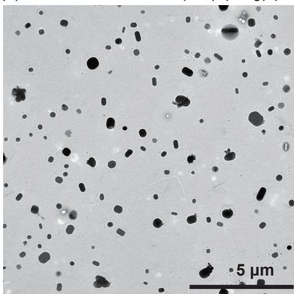
(b) Sulfate dominant sample (Summer) (10 August 2018)
