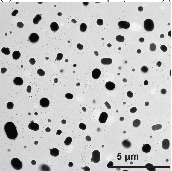
(c) Organic dominant sample (8 September 2017)
