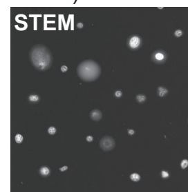
(c) Organic dominant sample (8 September 2017)
