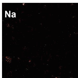
(c) Organic dominant sample (8 September 2017)
