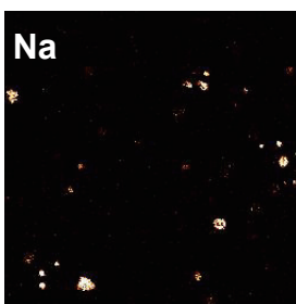
(b) Sulfate dominant sample (Summer) (10 August 2018)
