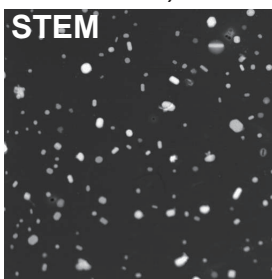
(a) Sulfate dominant sample (Spring) (15 March 2018)
