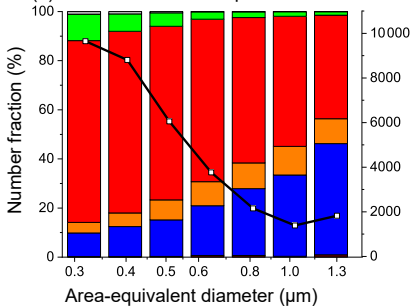
(a) Ambient aerosol samples
