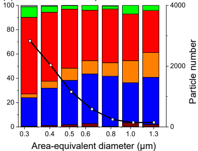
(b) Cloud residual samples
