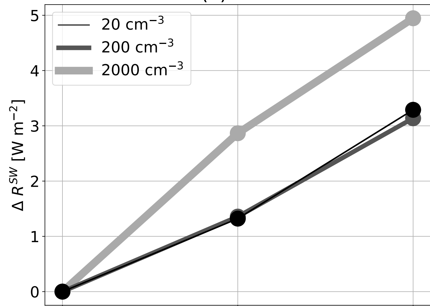
(a) R^{SW}
