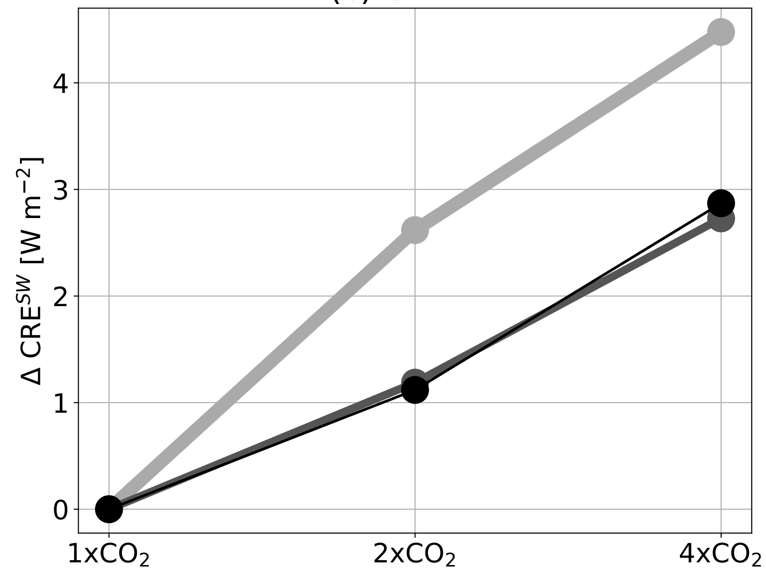
(c) \text{CRE}^{SW}
