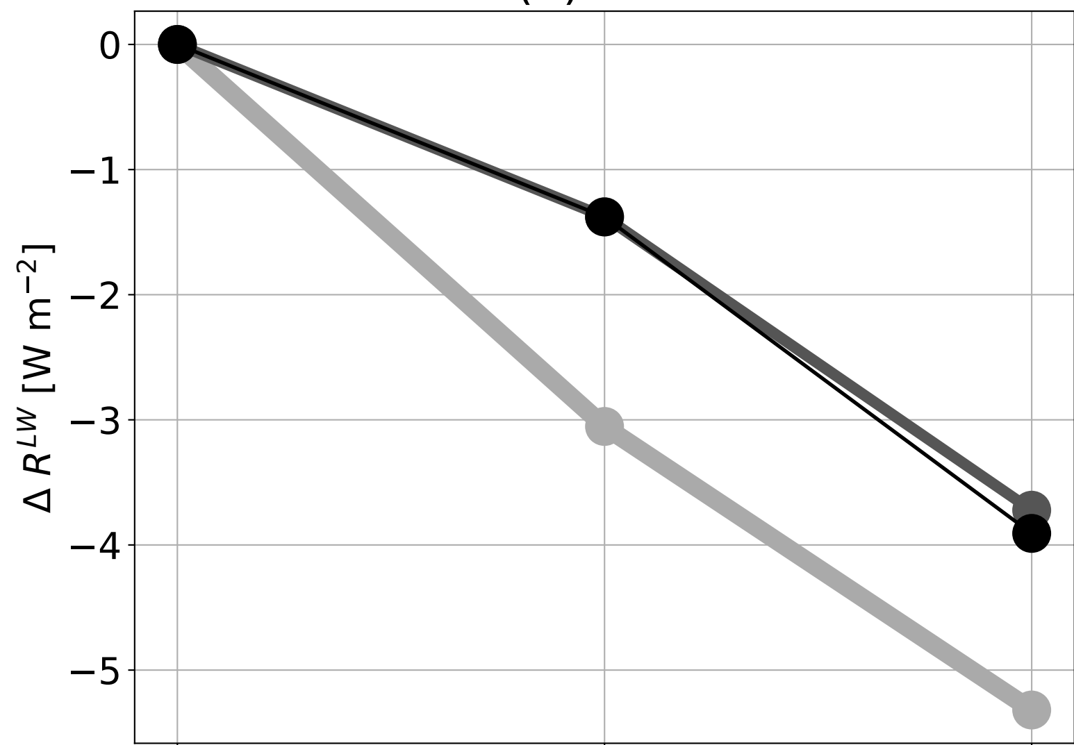
(b) R^{LW}
