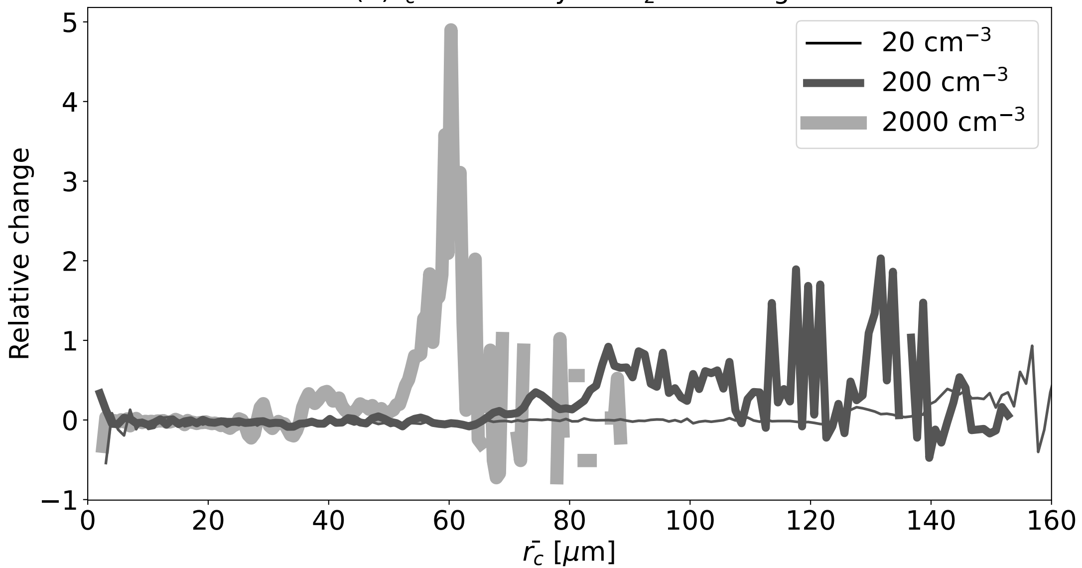
(b) \bar{r}_c sensitivity to CO 2 doubling
