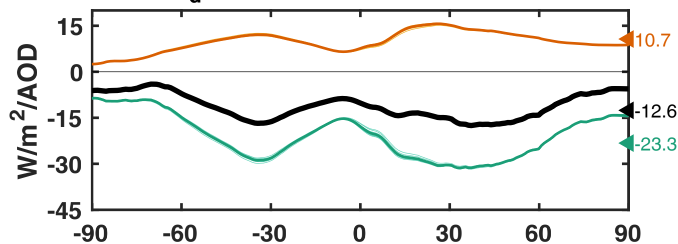
(c) \Delta F_d normalized to AOD [2081-2100]
