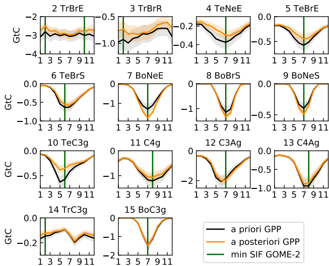
(a) GPP
