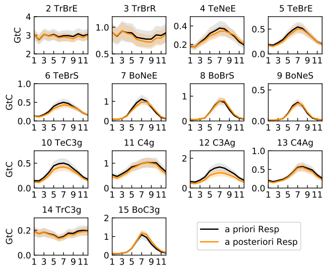
(b) Respiration
