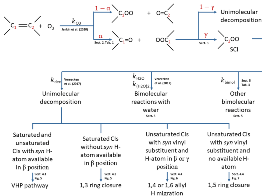
Figure 2. Flow diagram for implementation of the protocol. \alpha : branching ratios in POZ decomposition; \gamma : fraction of CI stabilised. > \text{COO} denotes the Criegee intermediate formed.
