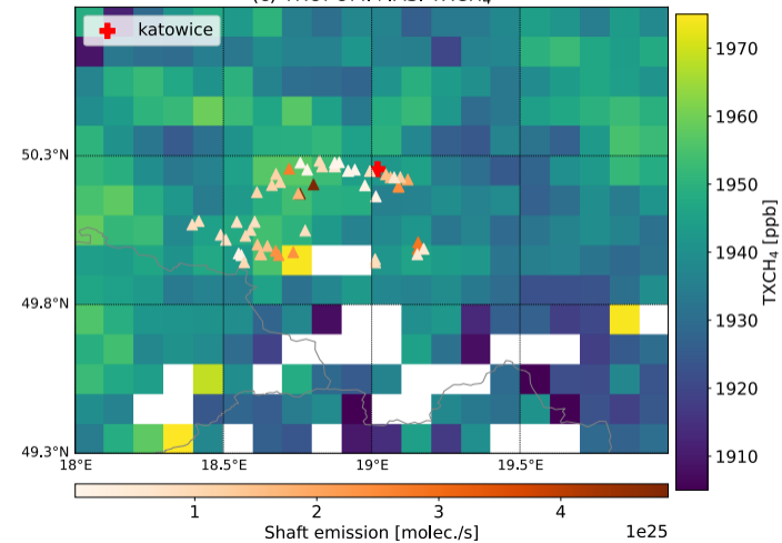
(c) TROPOMI+IASI TXCH 4
