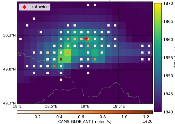
(a) CAMS forecast XCH 4
