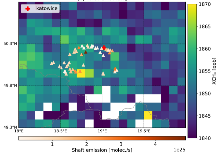
(b) TROPOMI XCH 4
