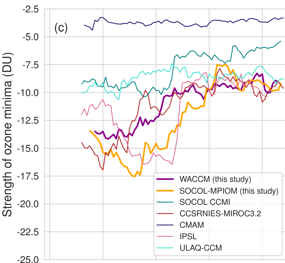
RCP2.6 - CCMI-1
