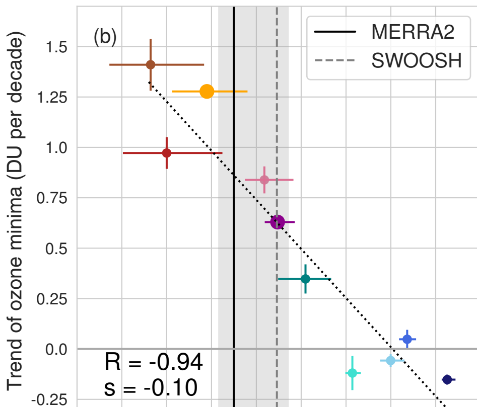
RCP8.5 - CCMI-1
