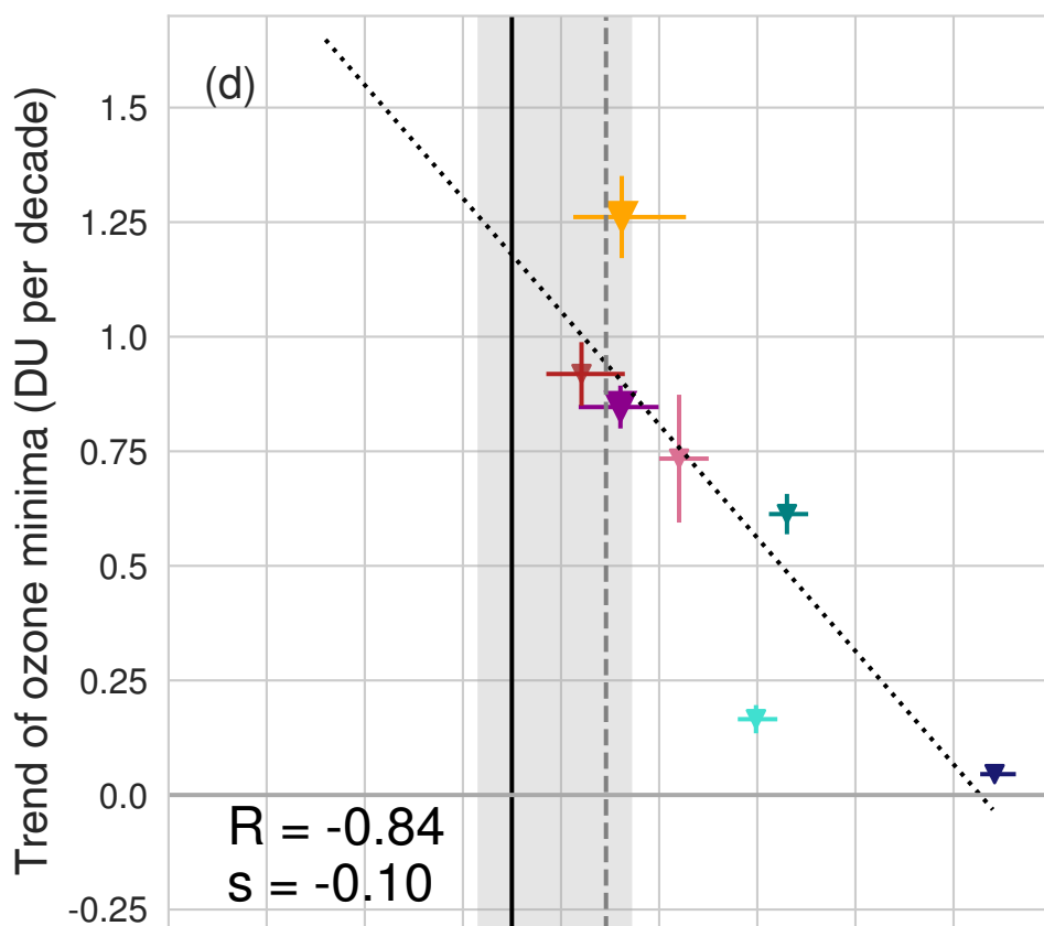
RCP2.6 - CCMI-1
