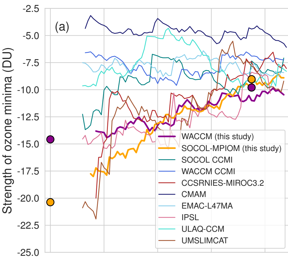
RCP8.5 - CCMI-1
