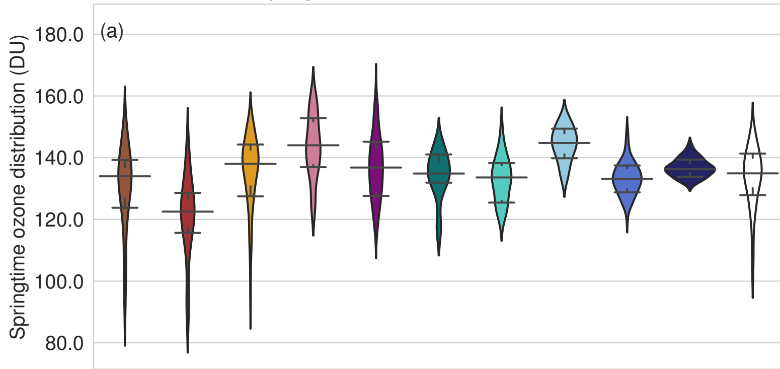
Springtime ozone distribution, 2005-2029
