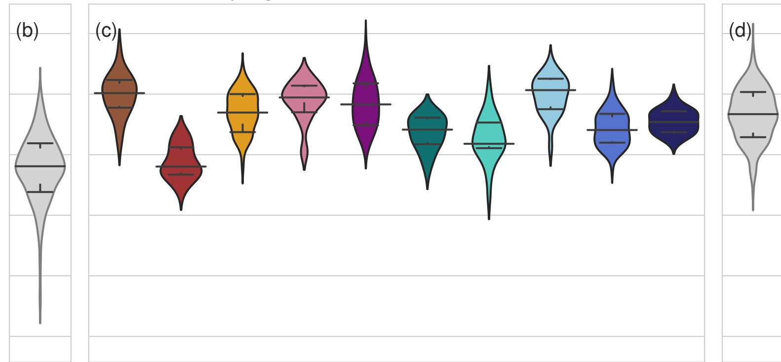
Springtime ozone distribution, 2070-2094
