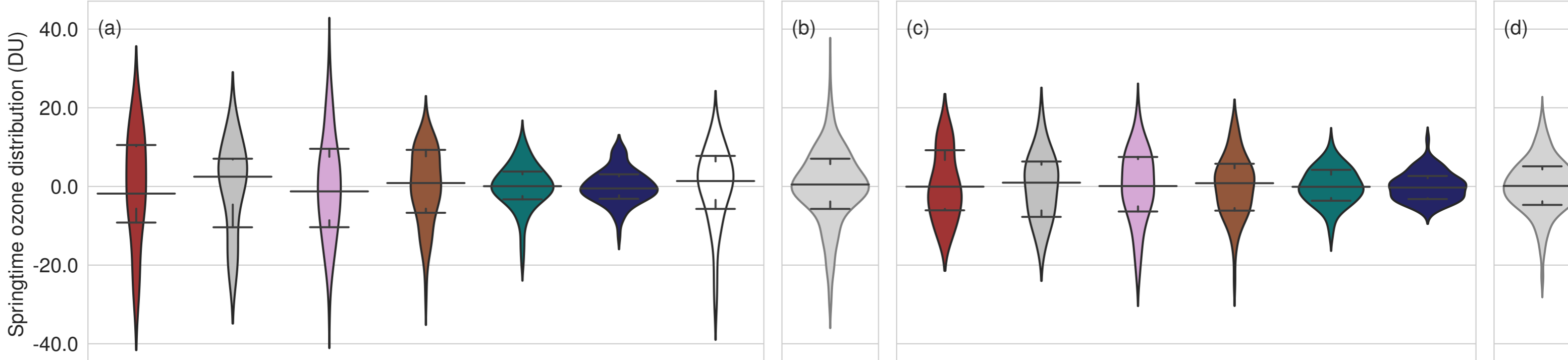
Springtime ozone distribution, 2005-2029
