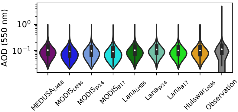
(e) AOD
