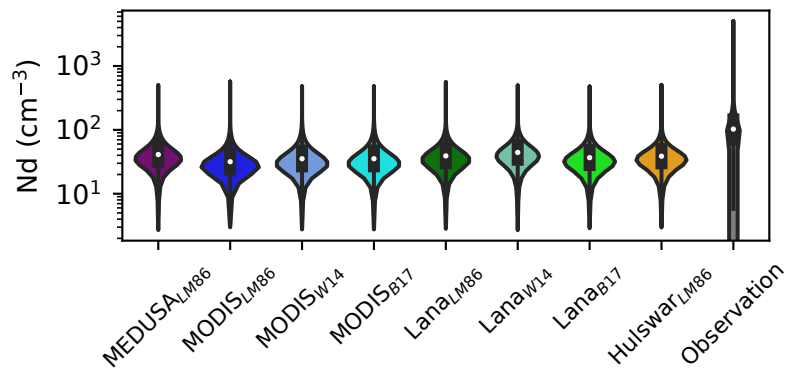
(c) CCN
