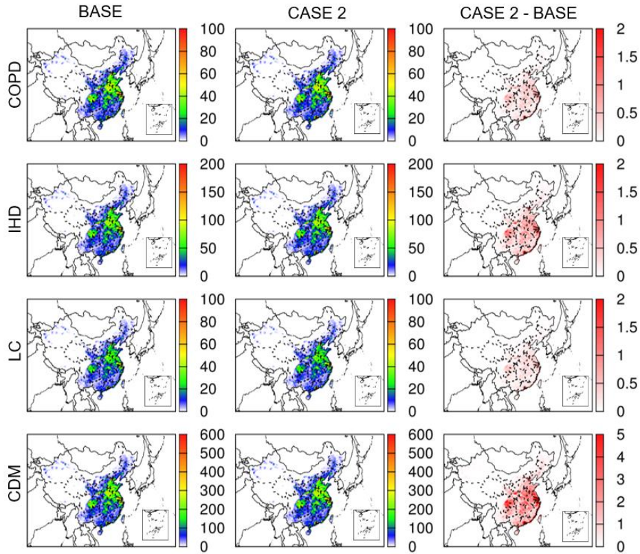
Figure S14. The O 3 -related premature mortality of (a) COPD, (b) IHD, (c) LC, and (d) CDM for BASE and CASE 2 and their differences.
