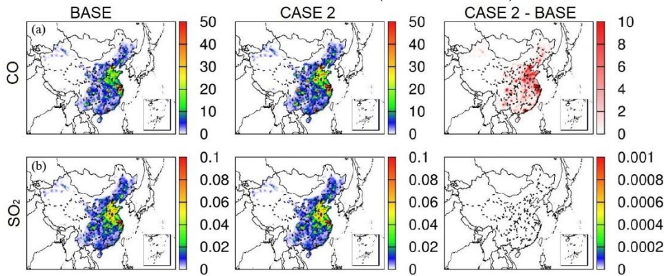
Figure S7. The annual average anthropogenic CO and SO 2 emissions of BASE and CASE 2, and their differences between these two cases (CASE 2-BASE) in 2020. Units are moles s -1 .
