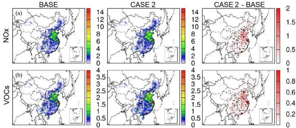
Figure S6. The annual average anthropogenic NO x and VOCs emissions of BASE and CASE 2, and their differences between these two cases (CASE 2-BASE) in 2020. Units are moles s -1 .
