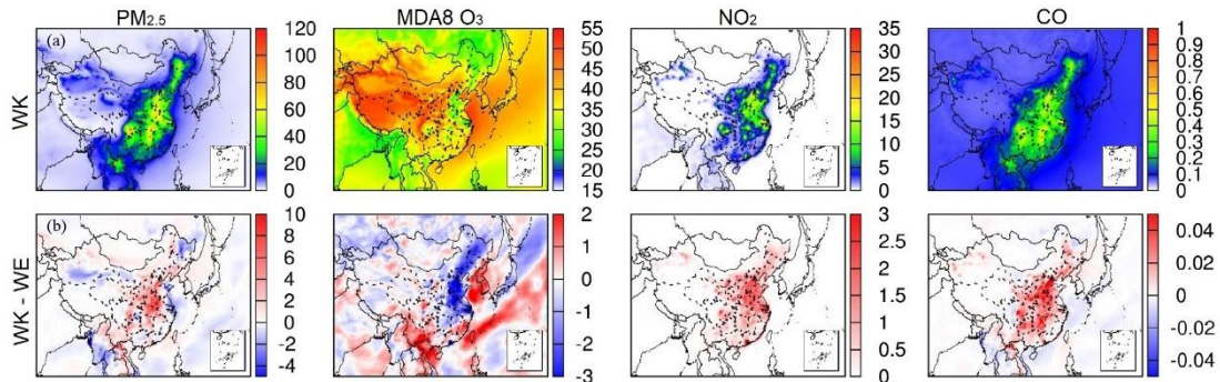
Figure S8. (a) is the concentration of PM 2.5 , MDA8 O 3 , NO 2 , and CO on workday (WK), and (b) is the differences of these pollutants between WK and weekend (WE) of CASE 2. Unit for PM 2.5 is μg m -3 , ppb for MDA8 O 3 and NO 2 , and ppm for CO.
