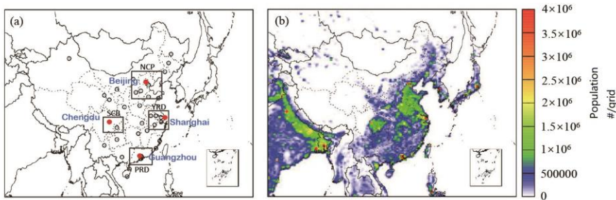
Figure S1. (a) is the CMAQ study domain and the key cities in China, and (b) is population data used in this study. For panel (a), red circle: cities in the TomTom data base, red dot: megacities (Beijing, Shanghai, Guangzhou, and Chengdu), black circle: other key cities in China such as the provincial capital.
