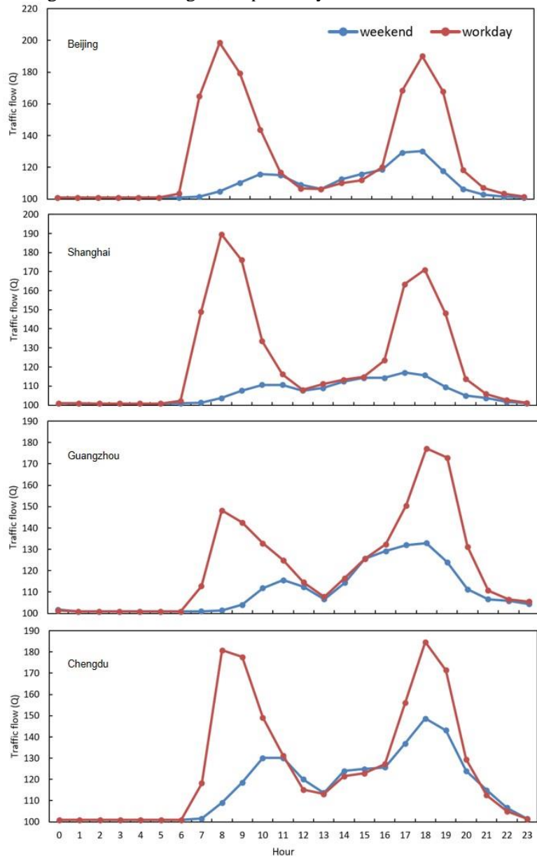
Figure S5. The hourly diurnal traffic flow calculated from TomTom congestion data in 2020 in Beijing, Shanghai, Guangzhou, and Chengdu, respectively.
