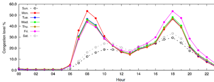
Figure S2. The 22-city average weekly congestion level (in %) from TomTom in 2020.
