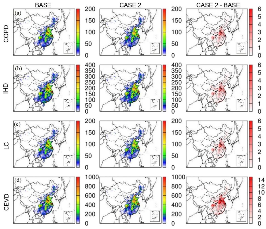
Figure S13. The PM 2.5 -related premature mortality of (a) COPD, (b) IHD, (c) LC, and (d) CEVD for BASE and CASE 2 and their differences.
