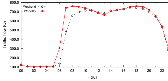
Figure S3. The 22-city average hourly diurnal traffic flow calculated from TomTom congestion data in 2020.
