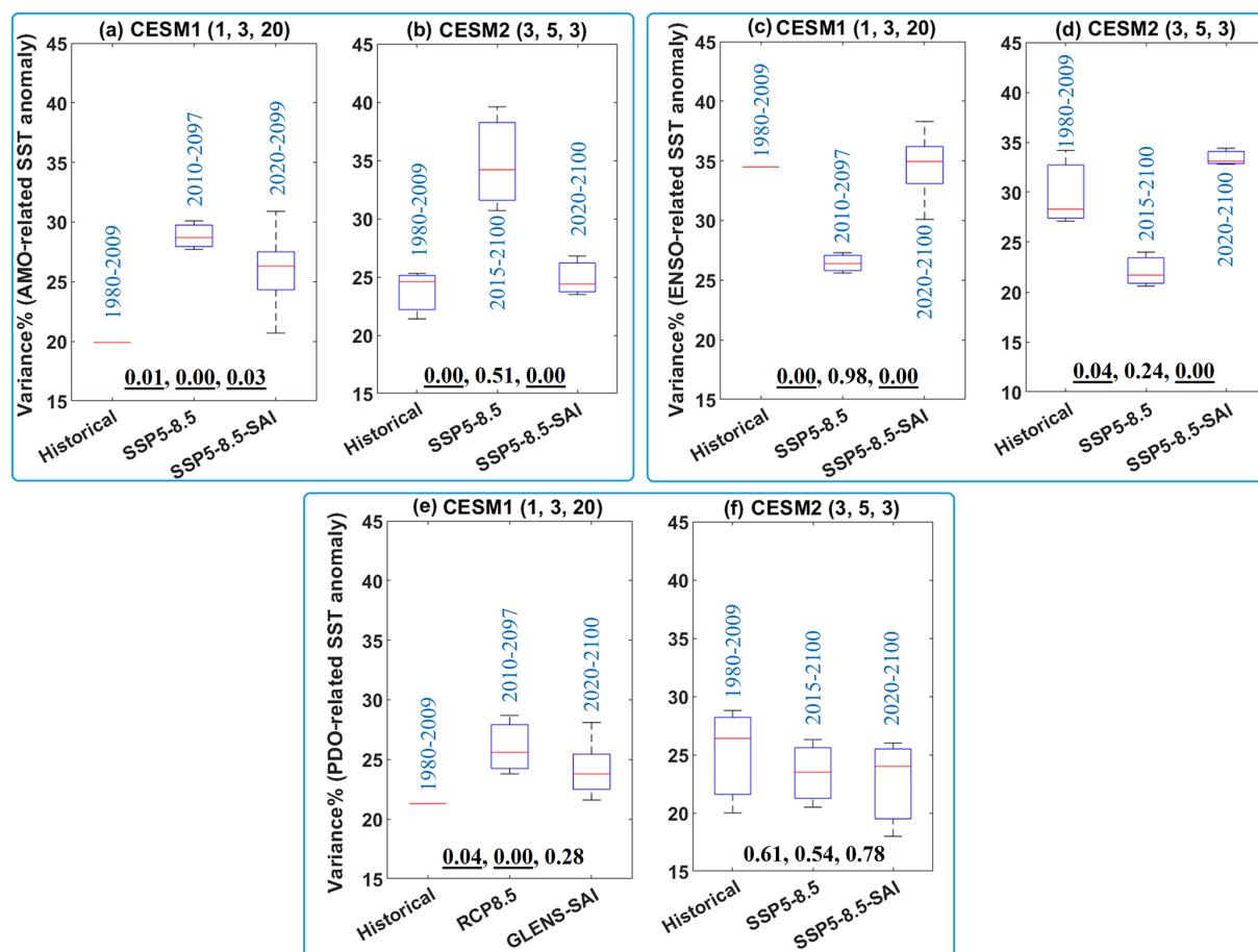
Figure 2. Box and whisker plots of the variance in the leading EOFs, representing the AMO, the PDO, and ENSO, relative to the total variance of the SST fields: the AMO across the North Atlantic (a, b), ENSO (c, d) global SST, and the PDO across the North Pacific (e, f). The values in blue in each column box show the period of the data for historical, GHG (i.e., RCP8.5 and SSP5-8.5), and climate intervention (GLENS-SAI and SSP5-8.5-SAI) scenarios. The titles of each subplot refer to the CESM version and the number of ensembles used in the historical, GHG (RCP8.5 and SSP5-8.5), and SAI (GLENS-SAI or SSP5-8.5-SAI) scenarios, respectively. The median for each experiment is denoted by the red line, the upper (75th) and lower (25th) quartiles by the top and bottom of the box, and ensemble limits by the whisker extents. The three values shown at the bottom of each subplot refer to the p values obtained from the statistical t test between historical and global warming, historical and SAI, and global warming and SAI, respectively. Values underlined are significant (i.e., p < 0.05 ).
