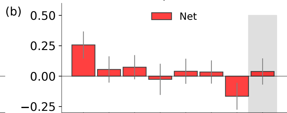
Unforced pattern effect
