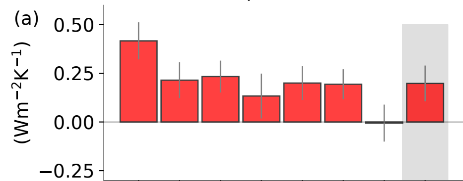
Total pattern effect
