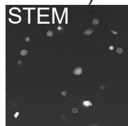
(e) 3 Sep 21:16 (agricultural smoke)
