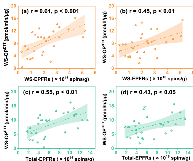
Figure 6. Correlation of WS-EPFRs and Total-EPFRs with WS-OP in \text{PM}_{2.5} : (a) WS-EPFRs with \text{WS-OP}^{\text{DTT}} , (b) WS-EPFRs with \text{WS-OP}^{\text{OH}} , (c) Total-EPFRs with \text{WS-OP}^{\text{DTT}} , and (d) Total-EPFRs with \text{WS-OP}^{\text{OH}} . The Pearson correlation coefficients ( r ) and associated p values are illustrated in the figure. The lines and shaded areas are linear regressions with their 95 % confidence intervals.
