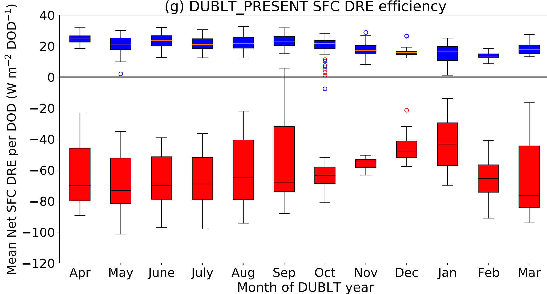
(g) DUBLT_PRESENT SFC DRE efficiency
