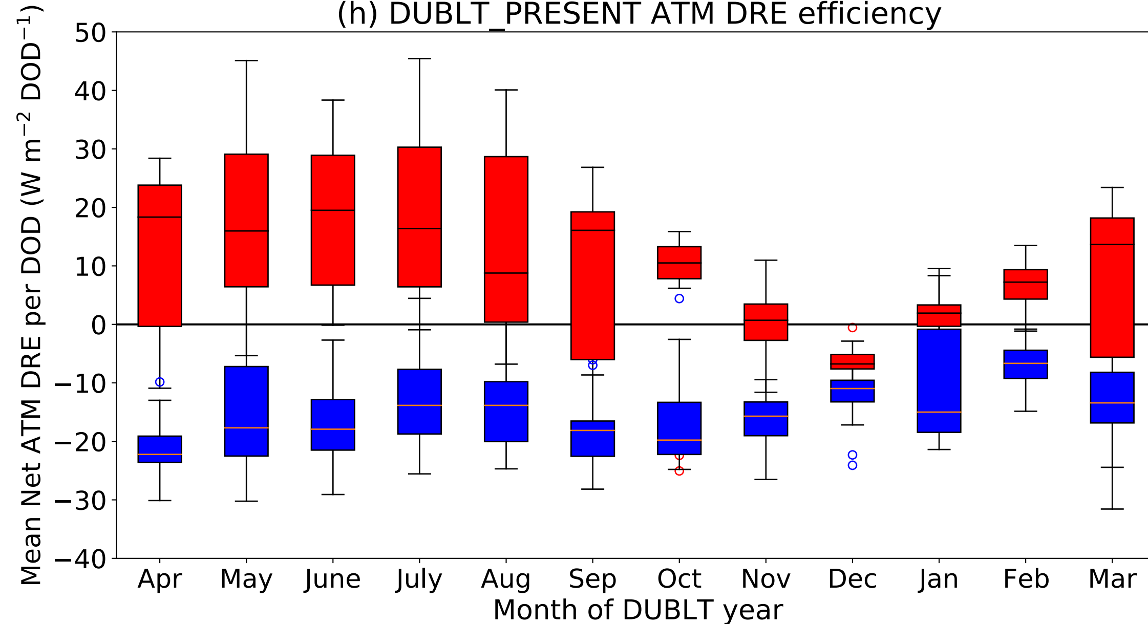
(h) DUBLT_PRESENT ATM DRE efficiency
