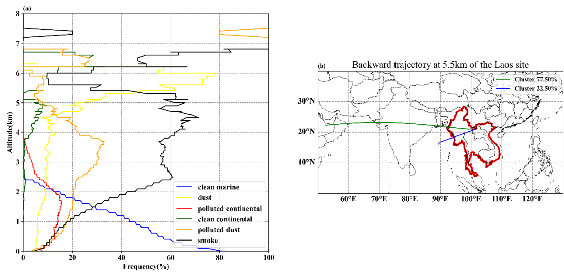
Figure. S4. (a) The frequency distribution of six aerosol types within an 8 km altitude over the PSEA region in March 2019 (the different colors represent the six aerosol types). (b) 48-hour mean backward trajectory air mass (5500 m) at the Laos site (20.93,101.41) in March 2019, where the red boundary is the PSEA region.
