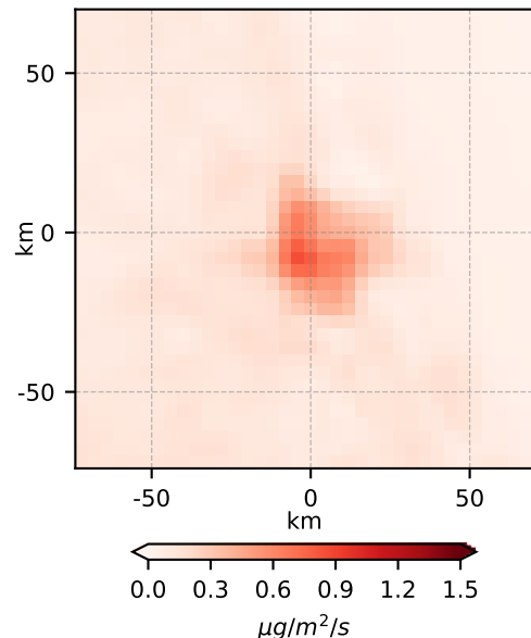
(c) derived NO x emission E_{NU-WRF}
