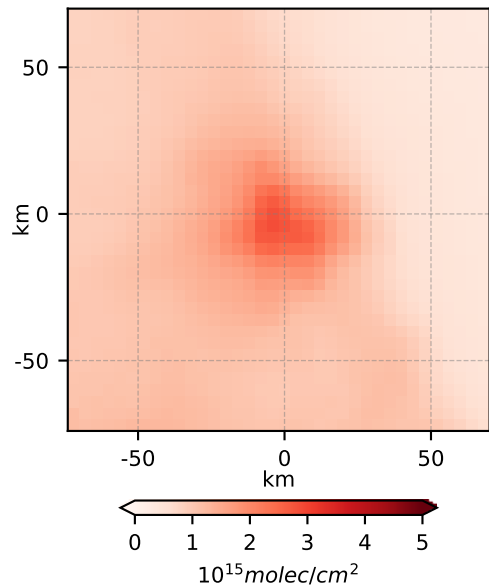
(a) NO 2 VCD
