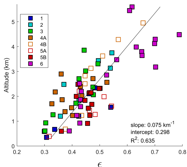
Figure 10. Profiles of DSD relative dispersion, \epsilon , for cases 1–6. Values of \epsilon are calculated locally at the measurement interval (1 s; \sim 100 m) and then averaged (weighted by N_d ) across a transect.
