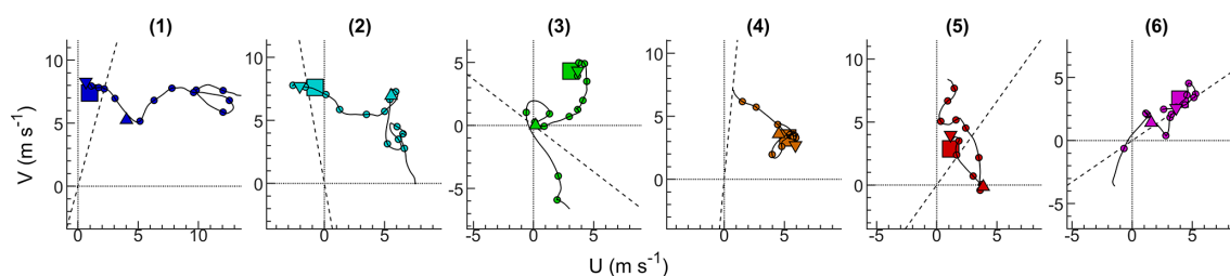
Figure 5. Case-mean dropsonde wind profiles displayed as hodographs for cases 1–6. The wind profile is smoothed with a 25 hPa running mean and markers (circle) indicate increments of 50 hPa. Also included are winds at cloud base (downward-facing triangle) and cloud top (upward-facing triangle; estimated based on the top of the Falcon module), the mean cluster motion from satellite imagery (square), and the primary axis of cloud organization estimated from satellite imagery (dashed line). In each panel the scale is preserved, with the position of the origin shifted to center the data. Case 5A dropsondes are omitted from (5) for readability but show a similar structure to case 5B (shown).
