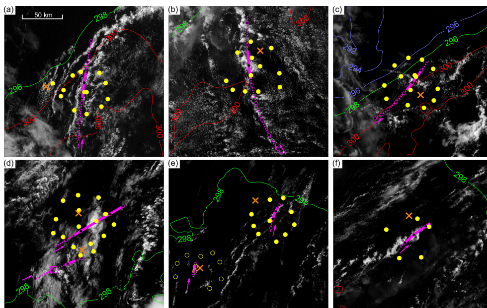
Figure 3. GOES-East ABI visible ( 0.6\ \mu\text{m} ) satellite imagery at the midpoint time of each process study. Panels (a–f) are cases 1–6, respectively, with a scale bar shown in panel (a). Overlaid on each panel – SST (K; contours), dropsonde locations (yellow dots), Falcon clear-spiral location (orange cross), and cloud cluster track (magenta). The cloud cluster track (see text) is separated into the time frame of the aircraft sampling (solid) and the remaining time window of the cluster lifetime (dotted). Hourly increments are shown as circles, and an adjacent arrow shows the direction of travel. Panels (d) and (e) are images from the midpoint of cases 4A and 5B, respectively. No dropsondes were associated with case 4B, but its cloud track is shown to the southwest of case 4A; the location of the tracked case 4B cluster at the time of the panel (d) image is marked with an open square. Dropsondes associated with case 5A are shown as open circles in panel (e), and the tracked cluster had already dissipated.
