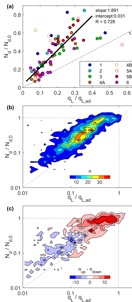
Figure 8. Variation in N_d and q_L with respect to a reference parcel with properties N_{d,0} and q_{L,ad} . (a) Transect in-cloud mean for cases 1–6 (open circles for secondary modules). A linear model is fit to the data using total least squares with equal uncertainty in q_L and N_d . (b) Joint frequency distribution (counts; n ) of all cloudy data for all cases with logarithmically spaced bins. (c) Same as (b) but showing the difference in the joint frequency distribution between updrafts and downdrafts.
