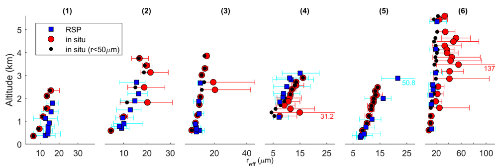
Figure 12. Comparison of the vertical profiles of effective radius, r_{\text{eff}} , for cases 1–6 between Falcon in situ cloud transects and composite profiles from RSP. The composite profiles were derived by grouping RSP retrievals into eight equal-frequency bins of cloud top height as determined by HSRL, with the mean altitude of each bin displayed. A comparison is made with in situ derived r_{\text{eff}} , omitting contributions from rainwater ( r < 50 \mu\text{m} ). For both datasets, the mean (markers) and 10%–90% range (bars) are shown.
