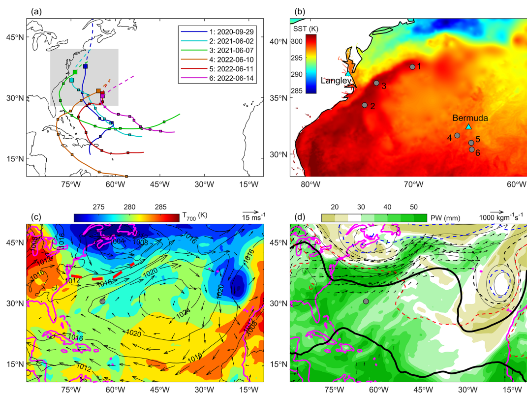
Figure 2. Large-scale meteorological environment. (a) 8 d back trajectory (solid) and 1 d forward trajectory (dashed) using MERRA-2 800–950 hPa layer averaged winds (see text) for cases 1–6. (b) Example SST shown for case 6 (14 June 2022) with all case locations shown for reference. The region in (b) corresponds to the grey-shaded region in (a) . (c) Case 6 sea level pressure (contours), 850 hPa wind vectors, and 700 hPa temperature (colored). The location of the axis of the stationary front (see text) is shown by the thick red dash. (d) Case 6 PW (colored), MF (vectors), 500 hPa geopotential height (contours at 6 dm – decameter, 10 m – intervals; thick contour designates the 588 dm level), and 1000–500 hPa thickness – dashed contours at 6 dm intervals; black contour designates the 564 dm thickness line; red (blue) contours represent regions of higher (lower) thickness.
