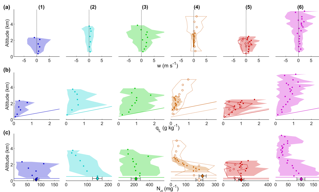
Figure 7. Statistics of in-cloud properties measured in situ for cases 1–6. (a) Vertical velocity, w ; (b) liquid water mixing ratio, q_L ; and (c) drop number concentration, N_d . The shaded region corresponds to the 10 %–90 % range, and dots are the transect mean values where data are filtered for clouds using q_L > 0.02 \text{ g kg}^{-1} . In the case of (a) , the transect means are calculated as a q_L -weighted mean referred to as w_L in the text. Also shown in (b) is an adiabatic parcel initialized from saturation at the lowest cloud base, shown as a horizontal line in (c) . Also shown in (c) is a reference aerosol concentration based on the particle number concentration exceeding 100 nm in diameter measured during sub-cloud sampling (marker – mean; bar – 10 %–90 % range). In (4) and (5), data for the secondary modules are included (case 4B and 5A, respectively) and are shown by dashed lines and open markers.
