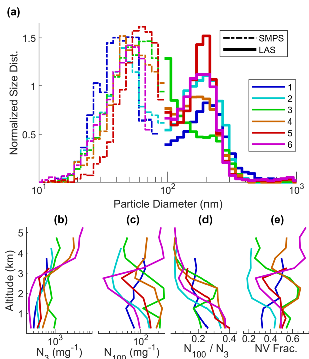
Figure 15. Aerosol microphysical properties for each case. (a) Normalized particle size distributions in the sub-cloud region and profiles of (b) total particle number concentration (> 3 nm), (c) total particle number concentration (> 100 nm), (d) the number fraction > 100 nm, and (e) non-volatile number fraction (> 10 nm).
