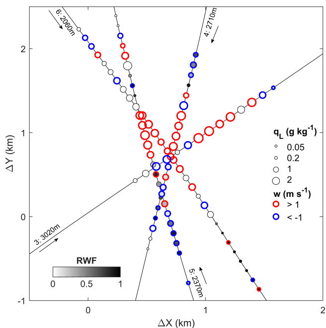
Figure 11. Four sequential Falcon in situ transects (2–3 km altitude) through a cloud during case 3. The aircraft position has been projected onto a cloud-centric coordinate where X(Y) represents the displacement along (perpendicular to) the cluster motion. The size of the markers corresponds to the total q_L , with shading indicating the rainwater fraction (RWF) defined as the fraction of q_L resulting from drop diameters exceeding 100\ \mu\text{m} . Red (blue) rings indicate updrafts (downdrafts).
