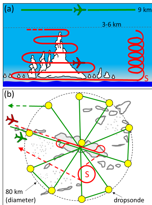
Figure 1. Schematic of the nominal two-aircraft flight strategy illustrating the position of the King Air (green) and the Falcon (red) (a) Cross section view of the altitude profile flown through the target cloud with adjacent clear spiral (S) and (b) plan view showing the “wheel and spoke” pattern.
