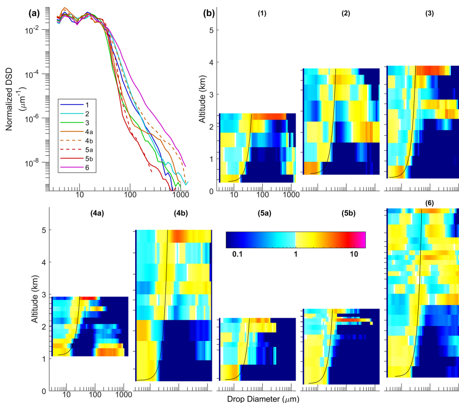
Figure 9. Vertical profile of the anomaly-normalized drop size distributions (DSD). (a) Reference normalized DSD calculated from the mean across all levels sampled. (b) For cases 1–6 at each level, the transect mean in-cloud DSD is normalized to unit integral, and then the anomaly is calculated as a ratio to the reference DSD. Warm (cold) colors therefore represent a higher (lower) than average contribution to the DSD shape, and use of the anomaly permits comparison across the size spectrum despite the large change in concentration. Also shown for each case is the monodisperse drop diameter of an adiabatic parcel (black line) initialized at the lowest cloud base with a drop number concentration, N_0 (see text).
