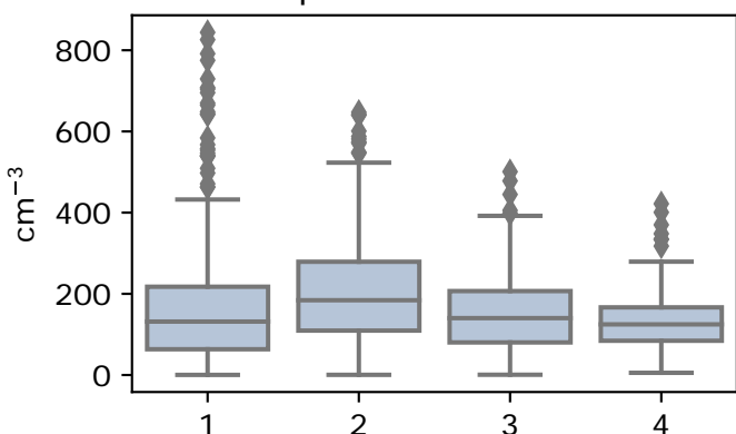
in-plume number concentration of activated particles at first cloud base
