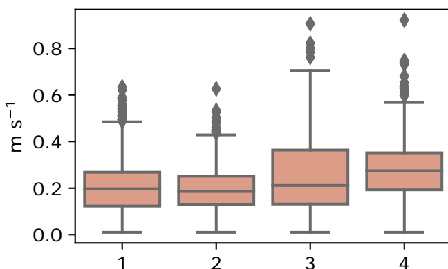
s.d. sub-grid updraft velocity at first cloud base
