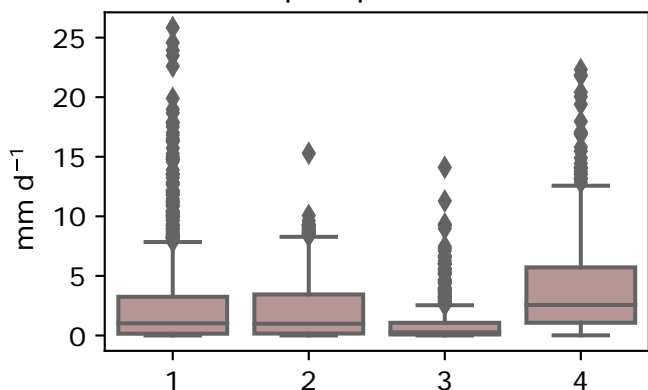
precipitation
