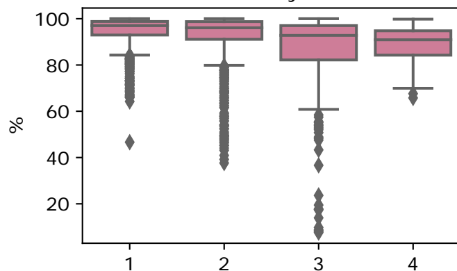
relative humidity at 950 hPa
