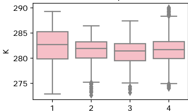
surface temperature
