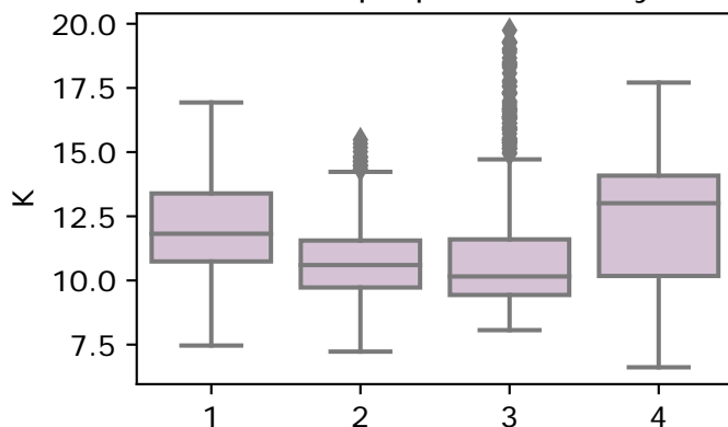
lower-tropospheric stability
