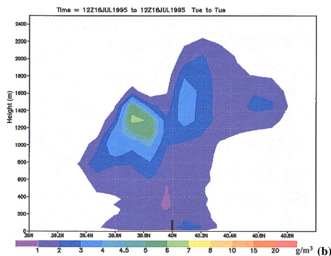
Fig. 10. Longitudinal cross section, spatially indicated in Fig. 2, of the simulated plume within grid G_2 for both meteorological simulations, S_1 and S_2 . Black line on lat. 40N indicates the power plant chimney height. (a) simulation S_{12} and (b) simulation S_{22} of the vertical distribution of the simulated \text{SO}_2 at Lon 0^\circ for 12:00 UTC on 18 July 1995. Under convective conditions with a well-developed sea breeze, the differences between the meteorological simulations of the PBL (Fig. 7) result in different mixing heights; thus, highly different plume fumigations on regions close to the point source are estimated.
