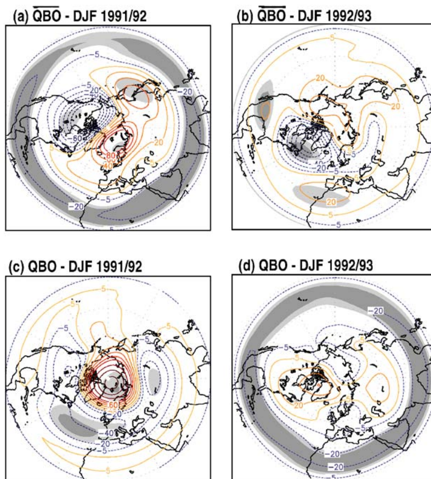
Fig. 3. Geopotential height anomalies (m) at 30 hPa for (a) QBO: DJF 1991/1992 (b) QBO: DJF 1992/1993, when the opposite QBO phase is prescribed; and for (c) QBO: DJF 1991/1992 and (d) QBO: DJF 1992/1993, when the observed QBO phase is prescribed. The shading denotes two levels (95% and 90%) of statistical significance in the order of lighter shading. Contours are at 20 m intervals until 100 m and then the intervals are at 40 m. A 5 m contour is added in the figures. The projection spans from 10 N to 90 N latitudinally.
