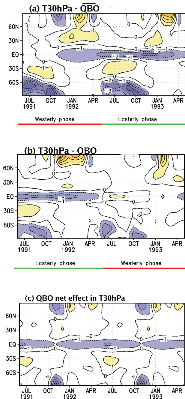
Fig. 2. Zonally averaged lower stratospheric temperature anomalies (K) at 30 hPa for two years following the eruption when (a) QBO is in the opposite shear (b) QBO is in the observed shear and (c) the climatological mean of the net QBO effect in zonal mean 30 hPa temperature (Punge and Giorgetta, 2008). The latitudinal extent is shown in the y-axis and is from 90S–90N. The anomalies in (a) and (b) are significant at >95% confidence level between 30N and 30S (not shown) and the winter anomaly north of 60N of October–November–December 1991 in (a) is also significant at >90% confidence level.
