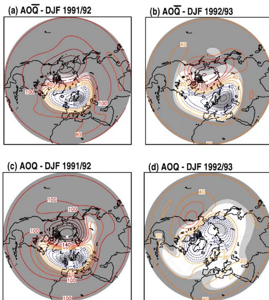
Fig. 5. Geopotential height anomalies (m) for (a) AOQ: DJF 1991/1992 (b) AOQ: DJF 1992/1993, when the opposite QBO phase is prescribed and for (c) AOQ: DJF 1991/1992 and (d) AOQ: DJF 1992/1993, when the observed QBO phase is prescribed. The shading denotes two levels (95% and 90%) of statistical significance in the order of lighter shading. Contours are at 20 m intervals up to 100 m and then the intervals are at 40 m. The projection spans from 10 N to 90 N latitudinally.
