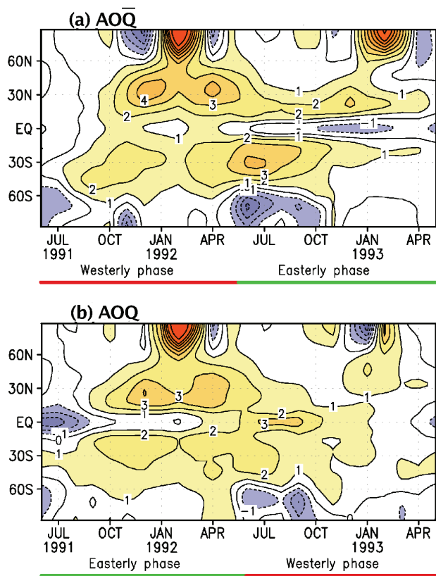
Fig. 4. Zonally averaged lower stratospheric temperature anomalies (K) at 30 hPa for two years following Mt. Pinatubo eruption for (a) AOQ with the opposite QBO phase and (b) AOQ experiment with observed QBO phase. The QBO phases encountered during (a) and (b) are shown by the colored lines. The anomalies within the 1 K contour interval in the latitudinal band of 60 N and 60 S is statistically significant at >95% confidence level (not shown). The winter anomalies north of 60 N are also significant at >90% confidence level for NDJFM of 1991/1992 and DJFM of 1992/1993 in (a) and for JFM of 1992 in (b).
