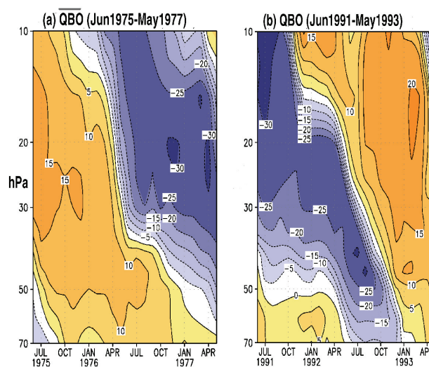
Fig. 1. Monthly averaged observed zonal mean zonal wind (m/s) at Singapore for (a) June 1975 – May 1977 and (b) June 1991 – May 1993. Negative values are shaded in colors of blue and are easterlies and the positive values are shaded in colors of yellow and are the westerlies. The contour interval is 5 m/s.
