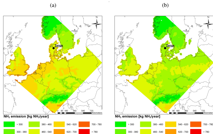
Fig. 2. Annual emission from storage in a reference pig production facility (located at Tange) with 1000 animals, when the facility is placed throughout central Europe and exposed to different European climatic conditions in the years (a) 2007 and (b) 2010.
