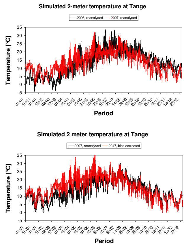
Fig. A1. (a) The hourly variation in simulated 2 m temperature for the Tange area that were used in the paper by Skjøth et al. (2011) and correspondingly hourly variations for the year 2006 using an identical model setup. (b) The hourly variation in simulated 2 m temperature for the Tange area that were used in the paper by Skjøth et al. (2011) and the simulated future variation on 2 m temperature using climate model output from the ENSEMBLES data set and bias correction.
