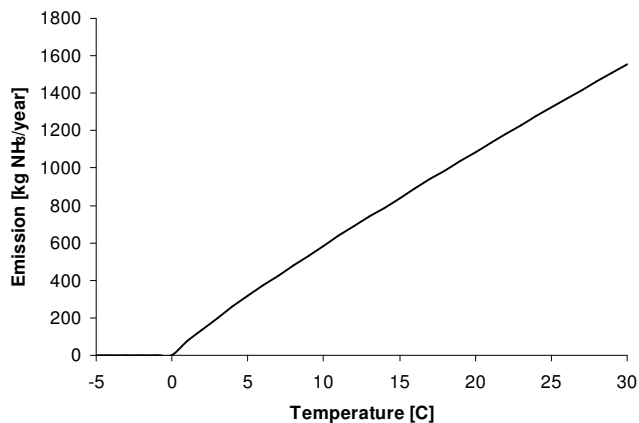
Fig. 1. Modelled annual ammonia emission from storage as function of temperature from a pig production facility with 1000 animals and production methods as in Denmark.
