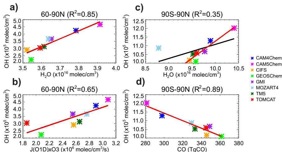
Figure 12. Annual mass-weighted tropospheric mean OH concentration as a function of the (a) annual mass-weighted mean water vapour concentration and (b) annual mass-weighted mean photolysis rates of J(\text{O}^1\text{D}) multiplied by \text{O}_3 concentrations in the Arctic, along with the annual mass-weighted global tropospheric mean OH concentration as a function of the (c) annual mass-weighted mean water vapour concentrations and (d) annual mean total tropospheric CO burden. The ordinary least squares (OLS) and the iteratively re-weighted least squares (IRLS) regression lines are shown in black and red, respectively. Correlations above 0.62 are significant at 90 % confidence level (CL) or above. Removing MOZART from analysis shown in (b) results in a r^2 value of 0.91, which is also significant above the 90 % CL. The troposphere has been selected according to the 150 ppbv \text{O}_3 contour, however, results are similar when using a climatological tropopause as described by Lawrence et al. (2001). The full list of regression coefficients (b) and coefficients of determination ( r^2 ) are shown in Table S1.
