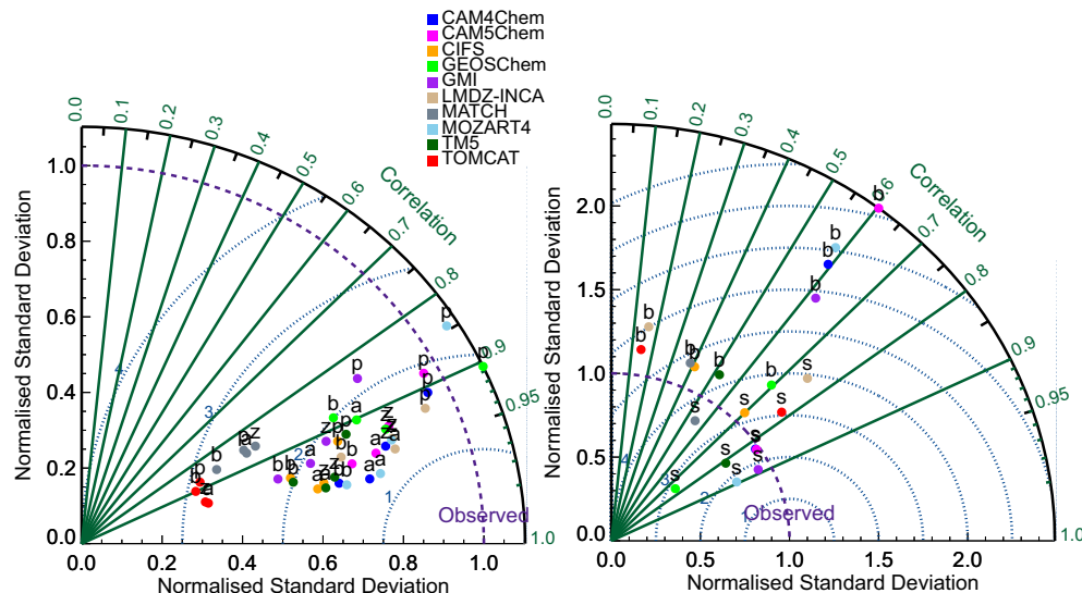
Figure 3. Taylor diagrams for Arctic surface comparisons of monthly mean time series of CO (left) and O 3 (right). Taylor diagrams show the extent to which models capture the observed variability (by the normalised standard deviation (NSD), shown by purple dashed contour), month-to-month changes in concentration (by the correlation ( r ), shown by green lines) and the mean model bias weighted by the monthly deviations from the annual mean (by the centered root-mean-square difference (RMSD), shown by the black dotted contours). Perfect agreement between a model and observations would result in a NSD of 1, a correlation of 1 and a RMSD of 0, which is indicated by “Observed” on the Taylor diagram. The letters represent the first letter of the station codes shown in Fig. 1.
