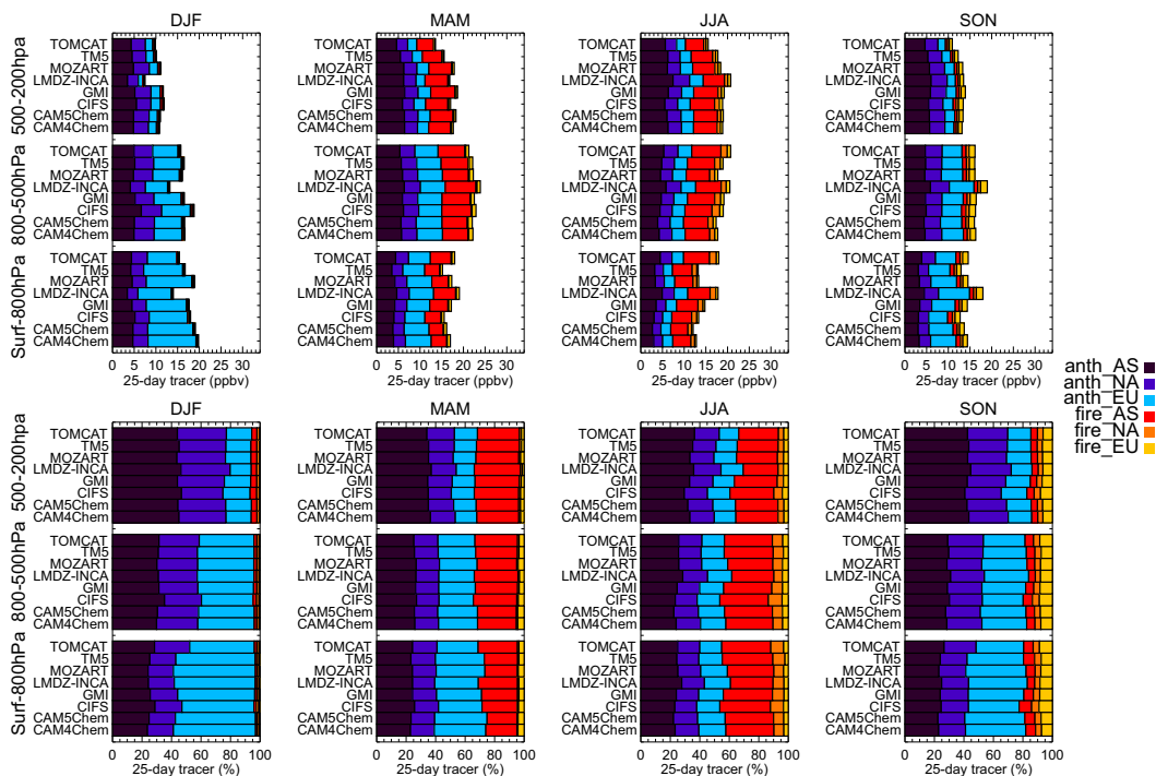
Figure 14. Seasonal mean 2008 regional 25 day fixed loss anthropogenic and biomass burning regional tracers averaged over 3 different altitude bands at latitudes north of 66^\circ N. Contributions shown as absolute concentrations (top) and as a percent of the total CO tracer (bottom). (AS = Asian tracer, NA = North American tracer, EU = European tracer).
