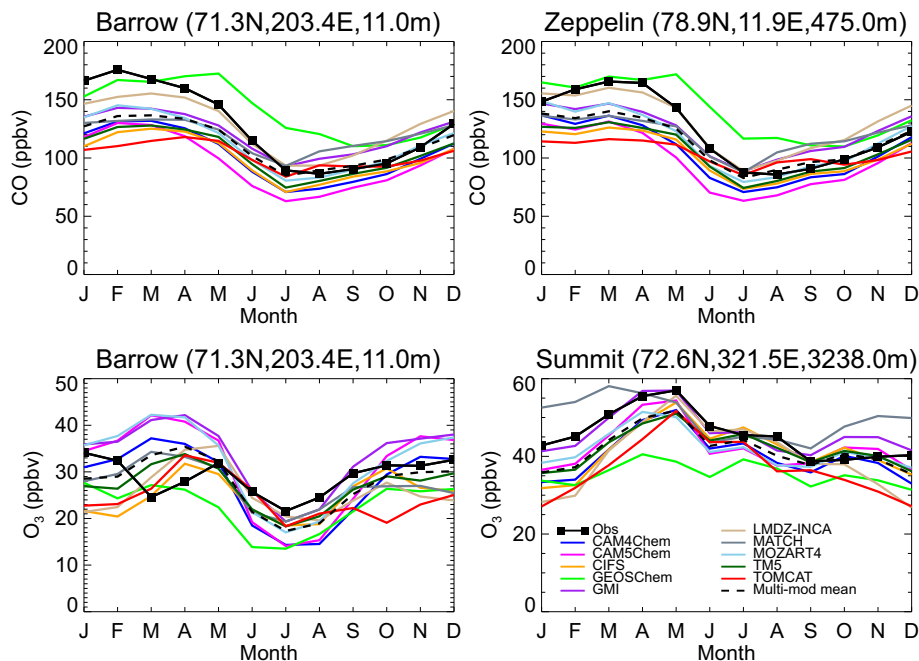
Figure 2. Monthly mean 2008 simulated and observed Arctic surface CO (top) at Barrow and Zeppelin and surface O 3 (bottom) at Barrow and Summit.
