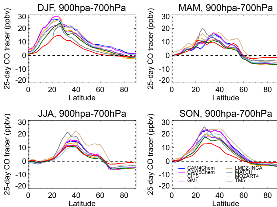
Figure 13. Seasonal zonal mean differences in simulated total 25 day fixed loss tracer (all six anthropogenic and fire tracers have been summed) between 900 and 700 hPa levels.
