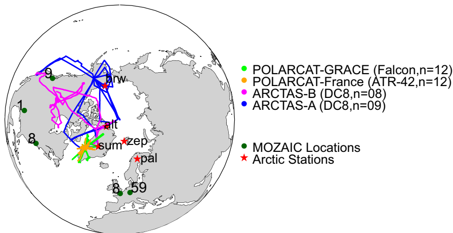
Figure 1. Location of surface stations used for comparisons in Figs. 2–3 (alt = Alert, brw = Barrow, pal = Pallas, sum = Summit, zep = Zeppelin), flight tracks of POLARCAT flights used to calculate vertical profiles in Figs. 7–8 (with n = no. of flights used) and locations of the airports where MOZAIC descent and ascent profiles were used over Europe and North America in Fig. 9 (the values denote the number of profiles at each airport).
