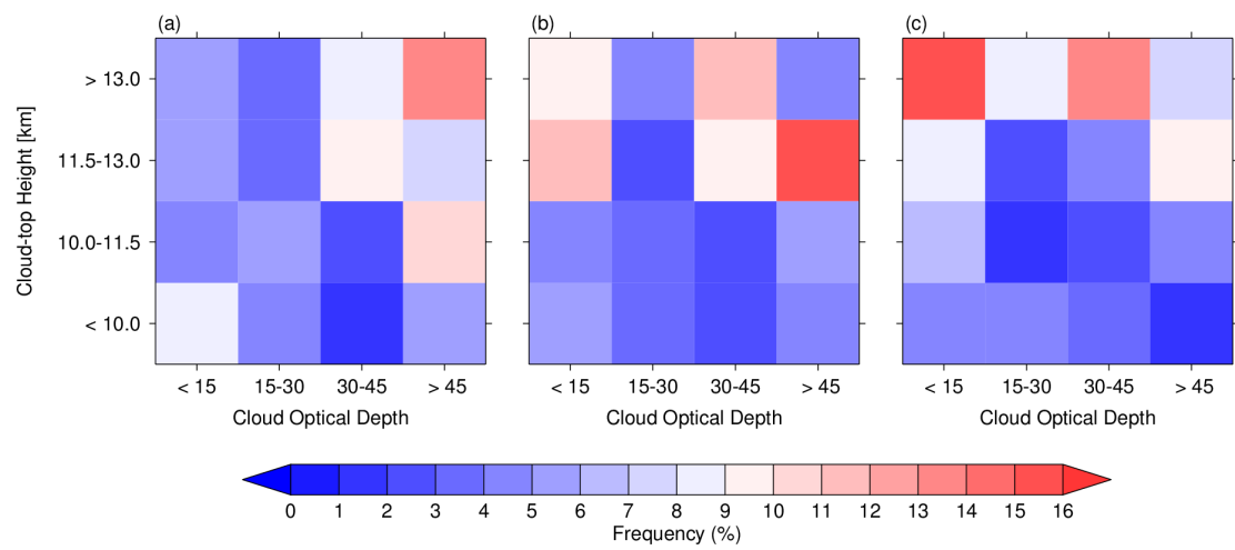
Figure 6. Cloud frequency of occurrence at three levels of CN concentration: (a) 0-2000 \text{ cm}^{-3} , (b) 2000-4000 \text{ cm}^{-3} , and (c) 4000-6000 \text{ cm}^{-3} . Data are binned according to COD and cloud-top height.
