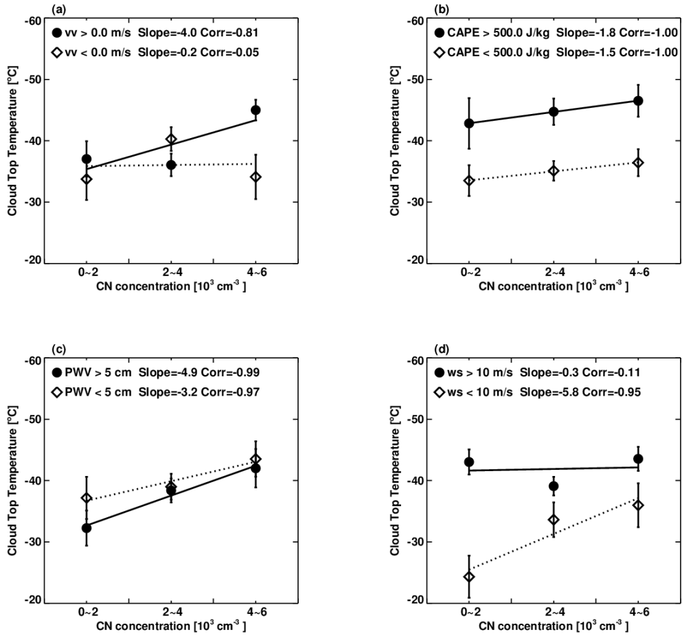
Figure 2. Cloud-top temperature as a function of aerosol CN concentration for deep convective clouds under different (a) vertical velocity (vv), (b) CAPE, (c) precipitable water vapor amount (PWV), and (d) wind shear (ws) conditions. Slopes and correlation coefficients of the different regressions are given.
