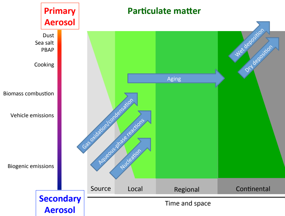
Fig. 1. Fig. 12 - Sources and processes affecting atmospheric aerosol composition from near-source to continental scales. The y-axis indicates the relative importance of primary vs. secondary aerosol for a given
