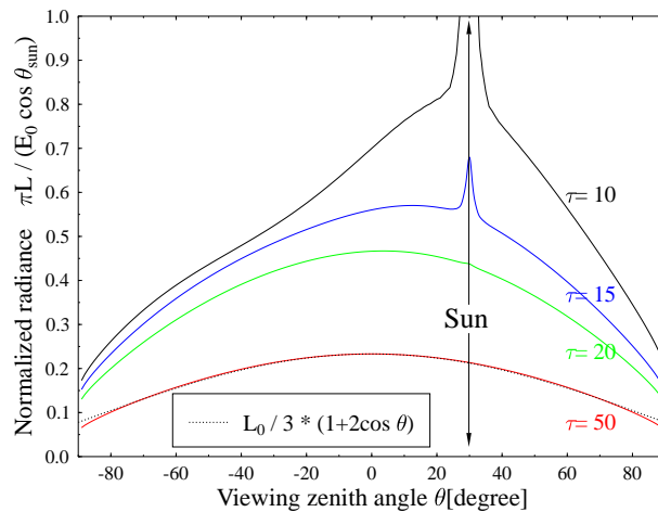
Fig. 14. Sky radiance distribution in the solar principle plane. The location of the sun at \theta_{\text{sun}}=30^\circ is marked. (Top) Rayleigh atmosphere. (Bottom) Cloudy atmosphere.
