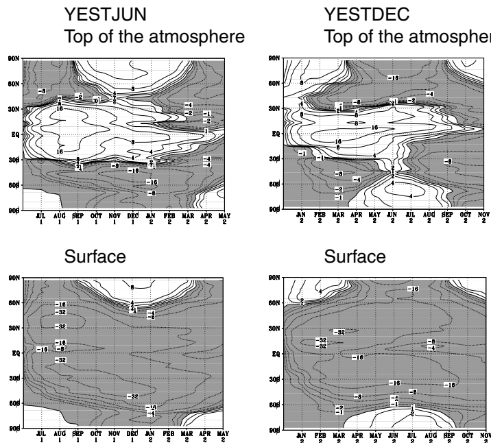
Fig. 5. Zonally averaged all-sky net radiative flux anomalies ( \text{W/m}^2 ) for YESTJUN (left panel) and YESTDEC (right panel) at the top of the atmosphere and at the surface. Numbers at the abscissae indicate month and year after the eruption.
