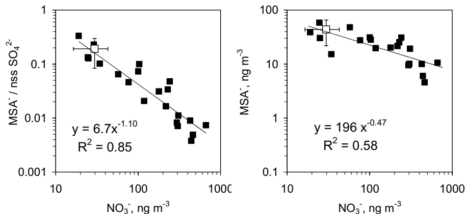
Fig. 10. MSA to nss sulfate ratio and MSA concentration as a function of nitrate concentration in HV samples taken over the ocean (closed squares) and at Aboa (open square). The error bars of the Aboa data point are the standard deviations.
