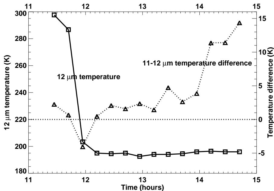
Fig. 1. Temporal evolution of the minimum 12 μm SEVIRI brightness temperature (solid line) for the Jebel at Tair eruption cloud. Also shown is the 11–12 μm brightness temperature difference (dashed line).
