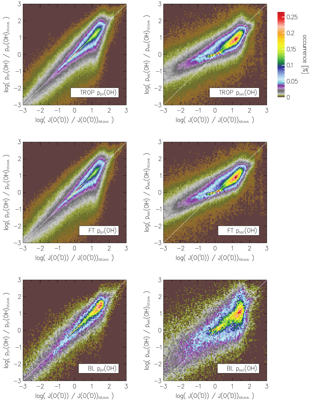
Figure 8: Correlation diagrams, showing P and S on the Y-axes as a function of the photo-dissociation rate of \text{O}_3 by R1, J(\text{O}^1\text{D}) , on the X-axes. Please notice the log/log scale. P is shown in the left panels and S in the right panels, in the 5 troposphere (top), FT (middle) and BL (bottom).
