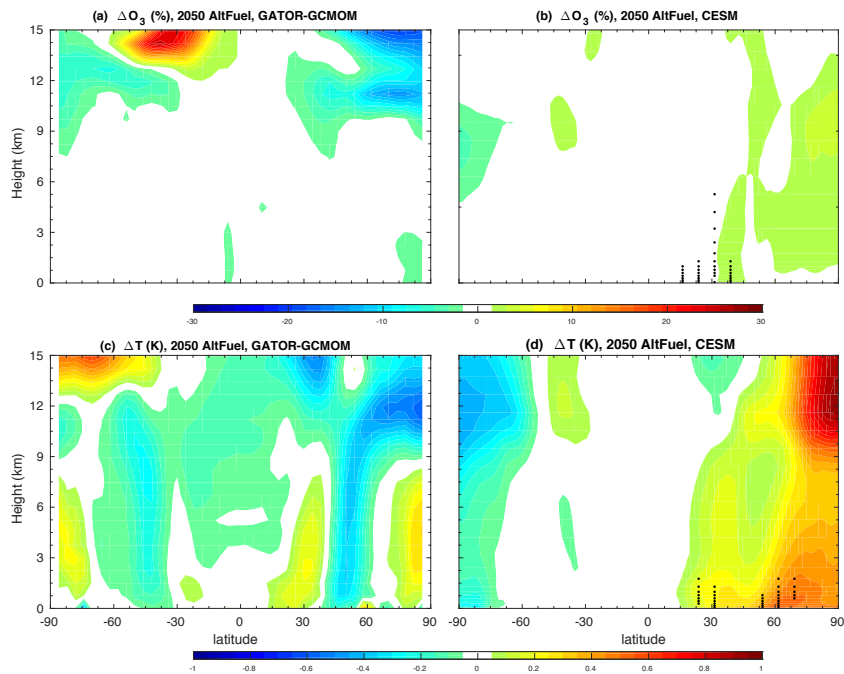
Figure 3: Zonal mean change in (A,B) ozone and (C,D) temperature due to Alternative Fuel 2050 aviation emissions (v. 2050 aviation emissions). Panels A,C for GATOR-GCMOM and B,D CESM. Black dots show regions of statistically significant
