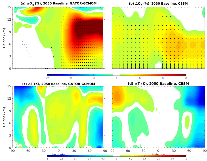
Figure 2: Zonal mean change in (A,B) ozone and (C,D) temperature due to baseline 2050 aviation emissions (v. no aviation emissions). Panels A,C for GATOR-GCMOM and B,D CESM. Black dots show regions of statistically significant perturbations using the False Discovery Rate method as described in the text. Based on first 5 years of simulations for GATOR-GCMOM, and years 31-50 for CESM.
