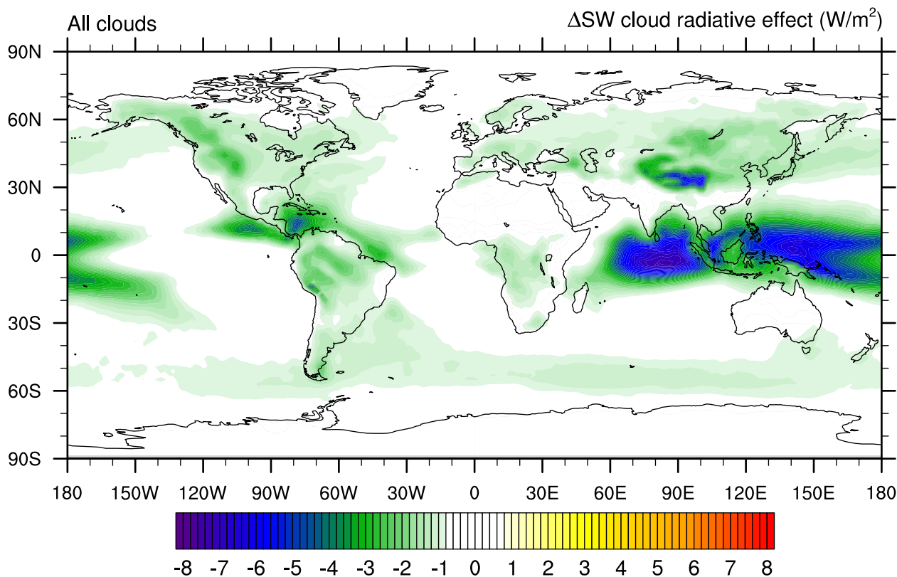
Figure 7. The global change in the shortwave cloud radiative effect predicted by the ECHAM-HAM model when the standard parameterization of the short-wave asymmetry factor is substituted by the parameterization using severely roughened ice particles. In this simulation the new short-wave asymmetry factors were applied to all ice particles both in cirrus and in mixed-phase clouds.
