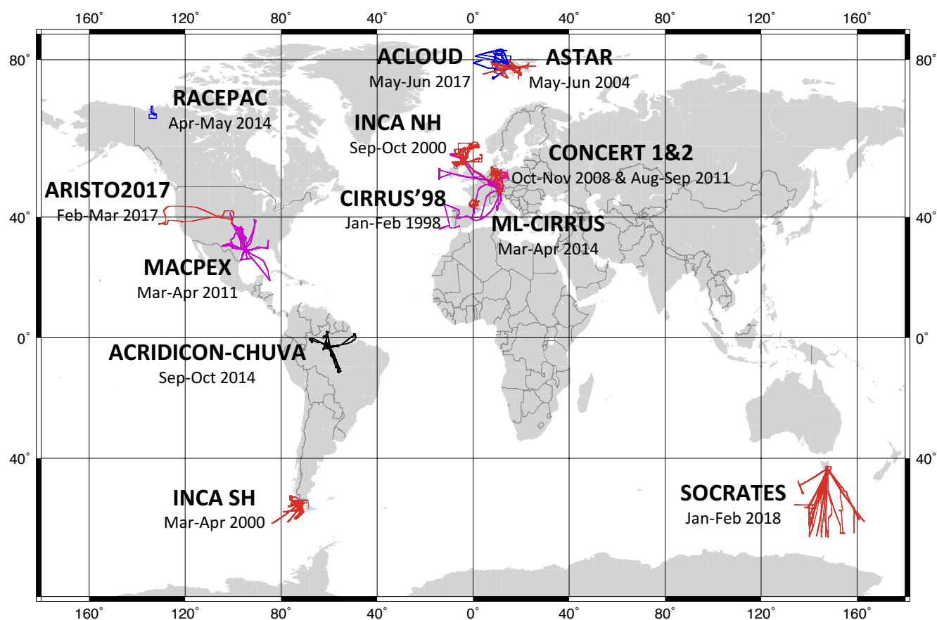
Figure 2. Flight trajectories of all campaigns included in this study. Trajectories of the campaigns where ice crystal submicron scale complexity was investigated are marked with black, purple and blue matching the colours used in Fig. 3. Trajectories of the campaigns where only angular light scattering function was measured are marked with red. Simultaneous submicron scale complexity measurements and angular light scattering measurements were performed in ACRIDICON-CHUVA and ACLOUD campaigns.
