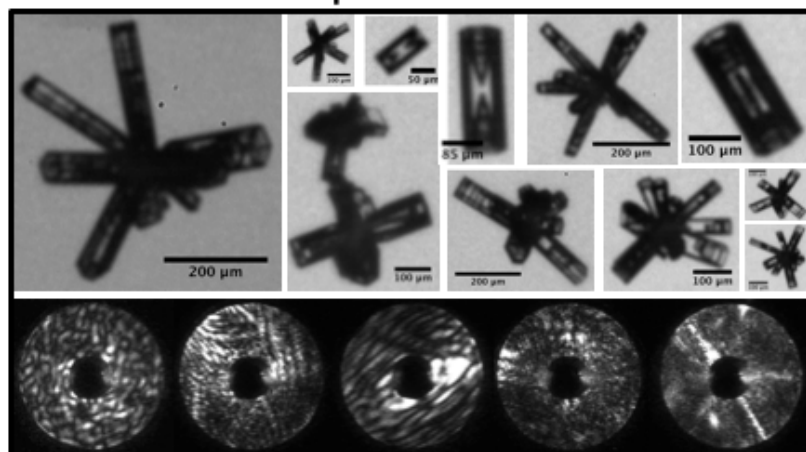
Figure 1. Hexagonal ice crystals and 2D diffraction patterns measured in laboratory simulations at -50^{\circ}\text{C} (upper panel) and in tropical cirrus at -60^{\circ}\text{C} (lower panel). The microscopic images of the laboratory produced ice crystals are from ice crystal replicas and the tropical cirrus ice particles were imaged in flight using bright field microscopy. The 2D diffraction patterns were measured simultaneously from the same particle population.
