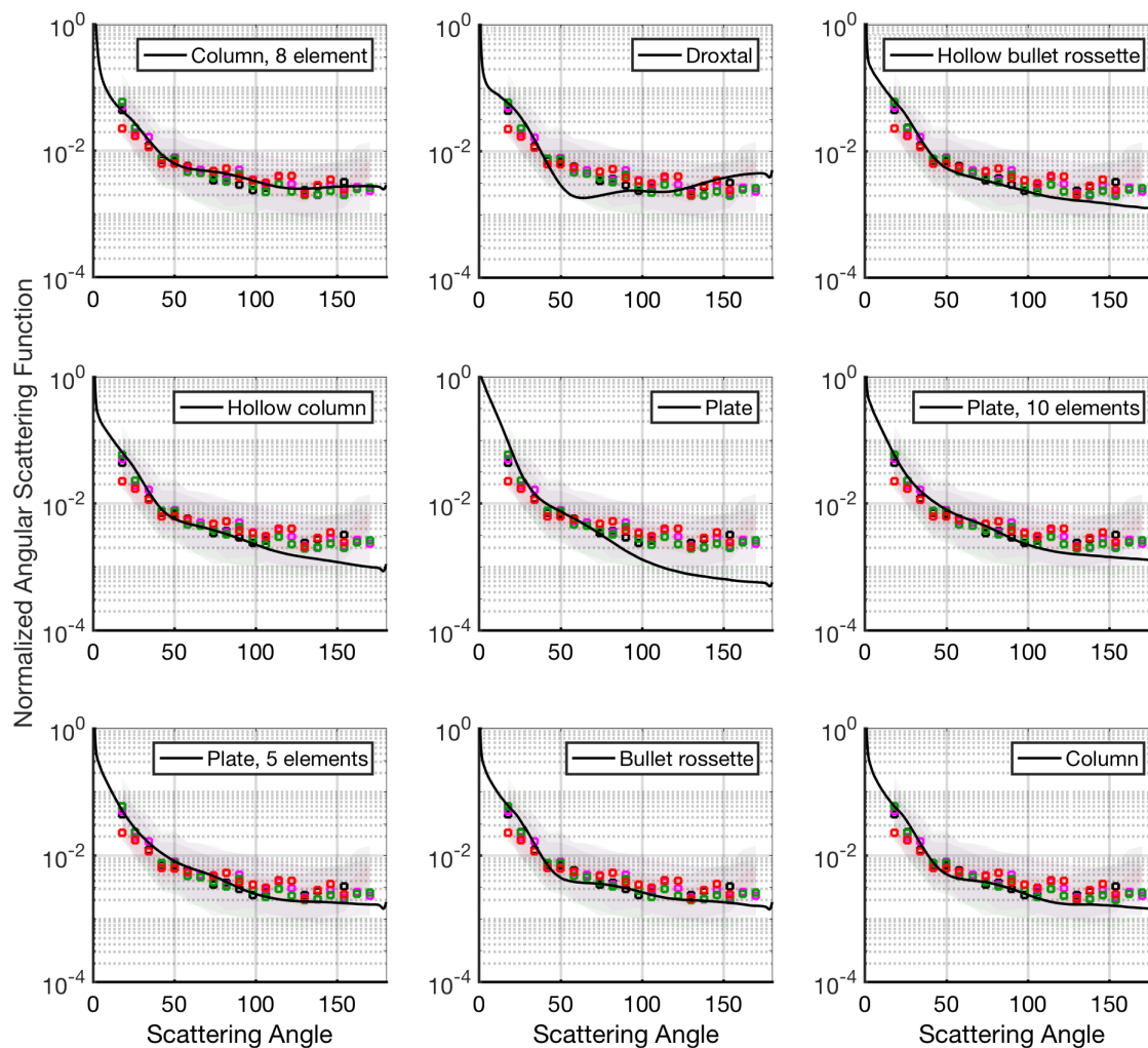
Figure 5. A comparison of the measured angular light scattering functions at 532 nm and different optical particle models from Yang et al. (2013). All models use severely roughened surfaces. Both the measurements and the model results are normalized to the total intensity between 18° and 170°.
