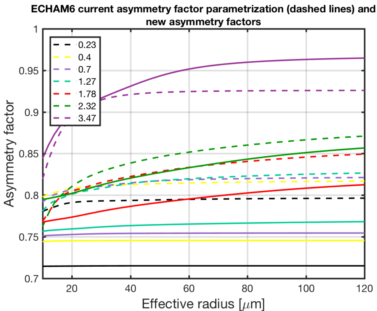
Figure 6. Comparison of the standard parameterization in ECHAM-HAM of the asymmetry factor of ice particle with different effective radius (dashed lines) and the new parameterization using severely roughened column aggregates (solid lines) for different wavelength bands. The wavelength bands are named with the band effective wavelength.
