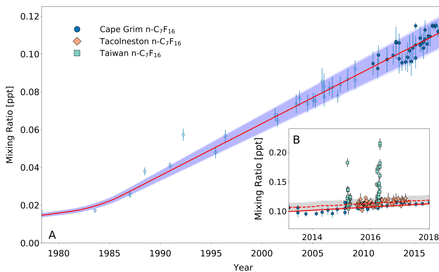
Figure 6. A) Mixing ratios at Cape Grim of n-C 7 F 16 between 1978 and 2018 (blue circles). Data prior to 2010 are shown as empty markers, while data from samples collected after 2010 are shown as filled markers to illustrate the part of the time series that is extended in the current work. Note that the data from Laube et al. have been converted to a new and improved calibration scale. The atmospheric trend simulated by the model is represented by the red line. Total uncertainties (light blue) and trend uncertainties (dark blue) are indicated with the shaded areas along the trend line. B) Mixing ratios after 2010 for Cape Grim (circles), for Tacolneston (diamonds), and Taiwan (squares). The red line indicates the modelled Southern Hemisphere baseline trend at Cape Grim, while the dashed red line indicates the modelled trend for mixing ratios at Tacolneston. Total and trend uncertainties are indicated with the shaded grey areas along the Tacolneston dashed-trend line.
