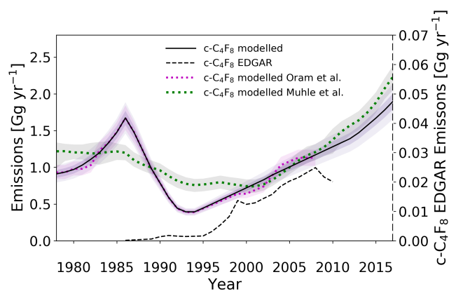
Figure 7. Estimated global emission rates for c-C 4 F 8 in this study (full black line), in Oram et al. (2012) (dotted magenta line), in Mühle et al. (2019) (dotted green line), and as reported in the EDGARv4.2 database (dashed black line). Note that the EDGARv4.2 emission rates are plotted on the secondary axis. Uncertainty envelopes include contributions from measurements, modelling, and calibrations.
