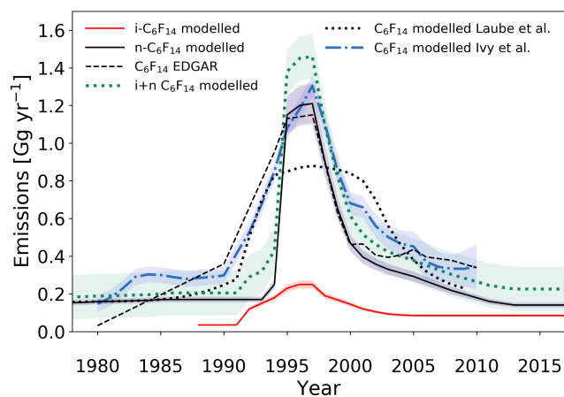
Figure 9. Estimated global emission rates for i-C 6 F 14 and n-C 6 F 14 in this study (full red and black lines, respectively), global emission rates for C 6 F 14 as reported in the EDGARv4.2 database (dashed black line; no distinction between isomers), by Ivy et al. (2012b) (dash-dotted blue line; no distinction between isomers), and by Laube et al. (2012) (dotted black line; no distinction between isomers). The sum of the global emissions for the isomers of C 6 F 14 , as reported in the current work, is illustrated by the dotted green line. Shadings illustrate uncertainties.
