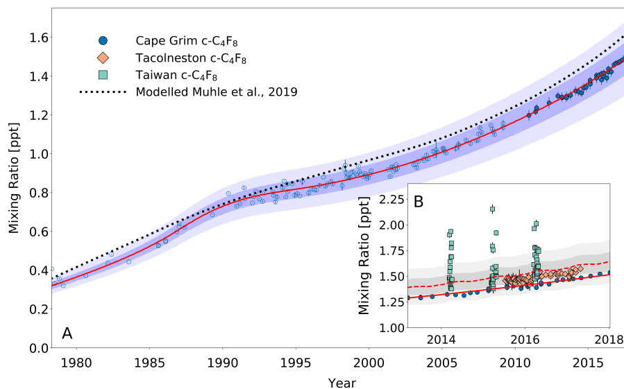
Figure 3. A) Mixing ratios at Cape Grim of c-C 4 F 8 between 1978 and 2018 (blue circles). Data prior to 2010 are shown as empty markers (Oram et al., 2012), while data from samples collected after 2010 are shown as filled markers to illustrate the part of the time series that is extended in the current work. The atmospheric trend simulated by the model is represented by the red line. Total uncertainties (light blue) and trend uncertainties (dark blue) are indicated with the shaded areas along the trend line. Results for the c-C 4 F 8 trend published in Mühle et al. (2019) are shown in the dotted black line. B) Mixing ratios after 2010 for Cape Grim (circles), for Tacolneston (diamonds), and Taiwan (squares). The red line indicates the modelled Southern Hemisphere baseline trend at Cape Grim, while the dashed red line indicates the modelled trend for mixing ratios at Tacolneston. Total and trend uncertainties are indicated with the shaded grey areas along the Tacolneston dashed-trend line.
