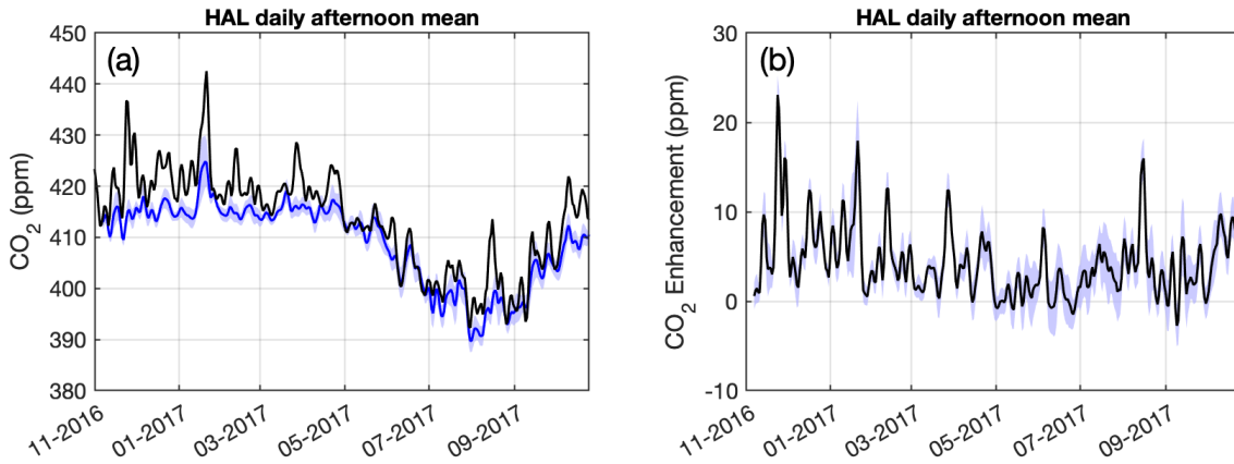
460 Figure 9. (a) Observed CO 2 time series at HAL for one year (black) with the background (blue) as the mean of five backgrounds from Table 1. (b) Corresponding CO 2 enhancement time series. We note that in summer the enhancements can be small or even negative, because they represent the impact of both positive (anthropogenic and biogenic) and negative (biogenic) fluxes in the urban domain. In both panels, lines are the 7-day moving average of mid-afternoon daily means; blue shading indicates the standard deviation of the five backgrounds.
