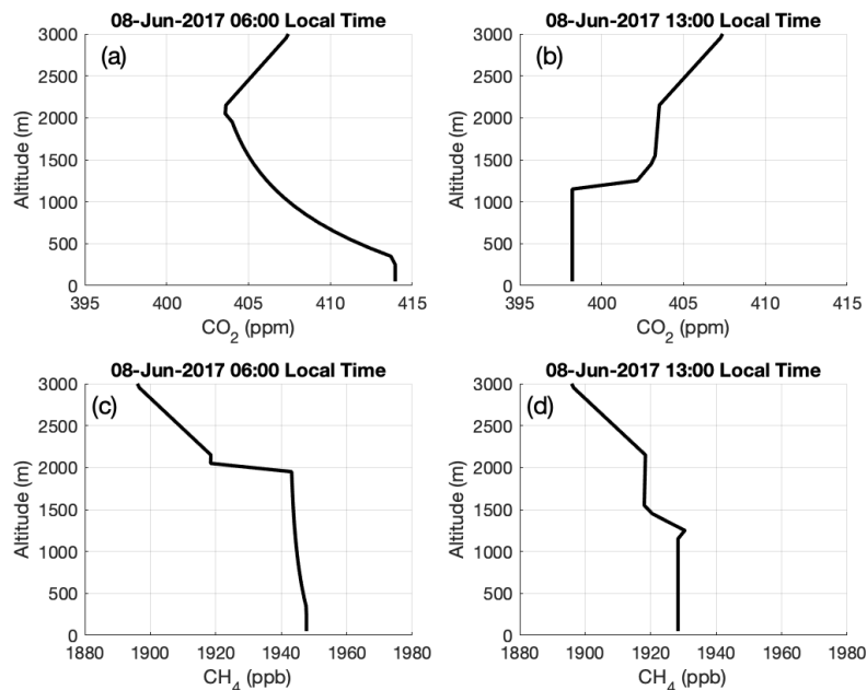
265 Figure 3. Examples of CO 2 (a, b) and CH 4 (c, d) vertical column profiles above BUC for morning (a, c) and afternoon (b, d) on a summer day with winds from the east (i.e., when the site is upwind of the urban domain). Profiles are constructed as described in the text.
