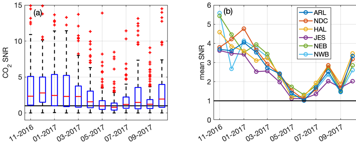
465 Figure 10. (a) Monthly box plot of the hourly signal to noise ratio (SNR) at all sites (afternoon hours only), calculated as the CO 2 enhancement ( y_{enh} ) above the background divided by the standard deviation of the backgrounds (Figure 8) for each hour. Red lines are medians; box edges indicate 25 th and 75 th percentiles; whiskers indicate the extent excluding outliers, which are shown in red + marks. The y-axis has been truncated for readability so some outliers, up to 30, are not shown. (b) Average SNR by month for each site. Black solid line in both panels indicates SNR=1.
