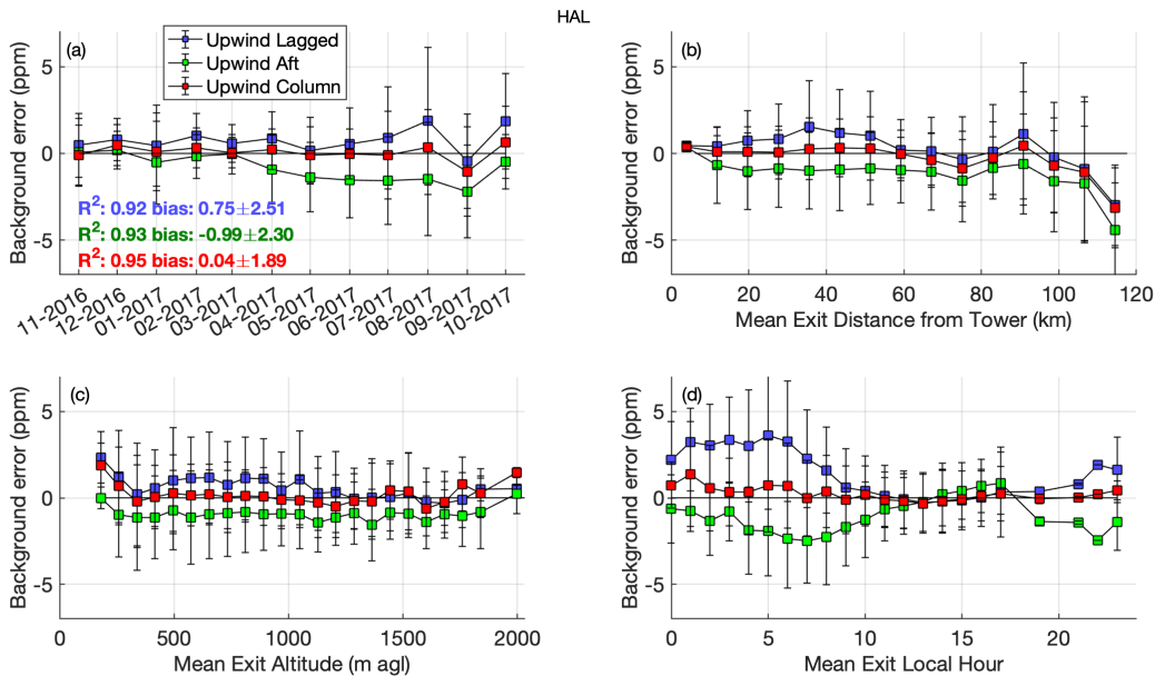
305 Figure 4. Results of the synthetic data study. Error in background (constructed background – true background) at HAL (afternoon hours only) for each method of using upwind site observations described in the text. Results for the other urban towers are similar. Red points indicate the column-based background (Upwind Col); green from sampling upwind sites at the same time as urban sites (Upwind Aft); blue from sampling upwind sites at the time of the particle exit (air mass entrance) earlier in the day (Upwind Lagged). Text in panel (a) indicates the coefficient of determination ( R^2 ) and mean bias \pm one standard deviation of the error over the entire year for each method in the corresponding colors. Panel (a) monthly mean, (b) binned by mean particle exit distance from the closest upwind tower, (c) binned by mean exit altitude, (d) binned by mean exit time of day. Error bars are standard deviations.
