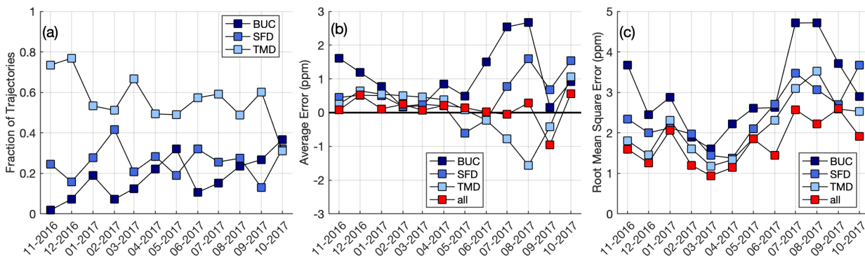
330 Figure 5. Results from synthetic experiment. (a) Fraction of STILT particle trajectories exiting closest to each background tower by month (MM-YYYY). (b) Bias and (c) RMSE for column-based upwind backgrounds (relative to the true background) in the synthetic data experiment using only a single background site (shades of blue), compared with the ideal scenario of all three background towers having available observations (red). Average values over the six urban sites for each month are shown.
