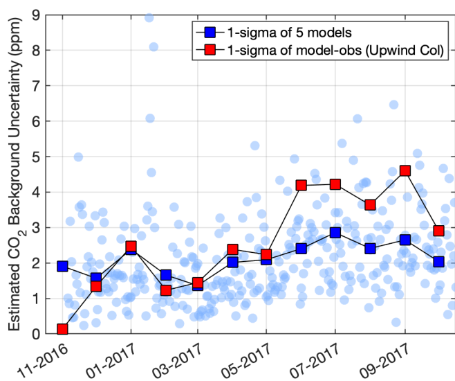
455 Figure 8. Comparison of two methods for estimating uncertainty on CO 2 background at HAL. The blue squares indicate monthly means of the standard deviation of five different backgrounds (light blue circles are daily). Red points indicate the monthly means of the standard deviation of the difference between modeled and observed mole fractions using the Upwind Column background during low-footprint periods. The other sites show identical patterns and very similar values.
