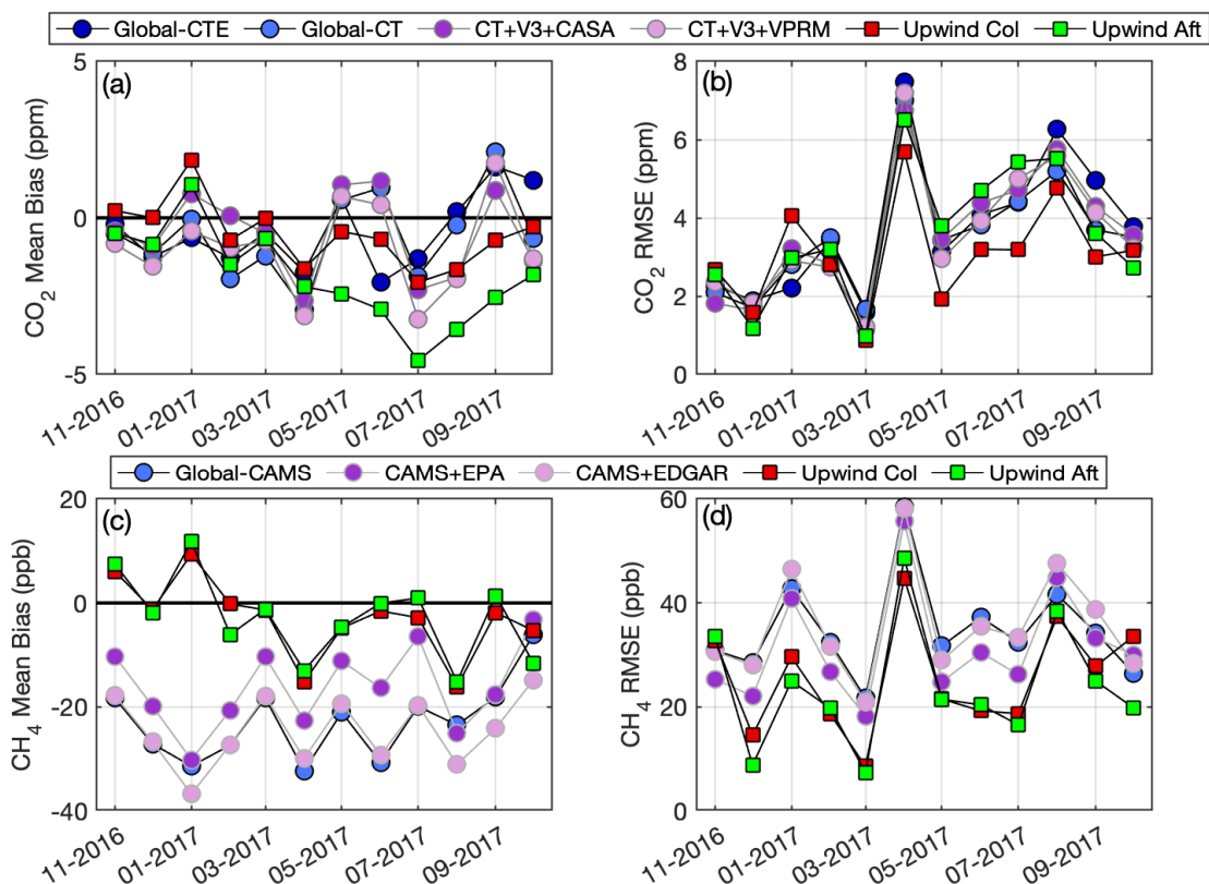
380 Figure 6. Average monthly bias (Model – Observations) (a, c) and RMSE (b, d) for different backgrounds over all six urban sites during periods of low influence from within the domain of interest. (a, b) are for CO 2 ; (c, d) are for CH 4 . All models use the same fluxes inside the urban domain; only the background varies, as indicated in the legends above each set of panels, with abbreviations from Table 1.
