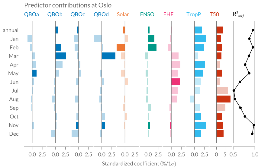
Figure 6. Predictor contribution to the regression fit at Oslo for the full annual regression fit and individual monthly fits. The standardized coefficients describe the percentage change in ozone for a 1-standard-deviation change in the predictor. Pale color bars indicate that the predictor’s contribution to ozone is not significant ( p -value of the coefficient < 0.05 ). The last panel on the right shows the adjusted coefficient of determination ( R^2_{adj} ) for the annual and all monthly fits. Note that the range of the x-axis is different for T50 than for the other predictors.
